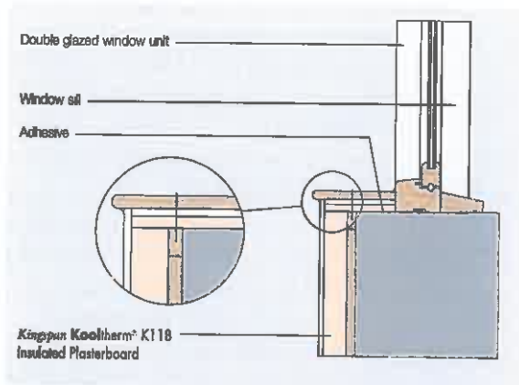
Figure 11 – Insulated reveal and external corner
