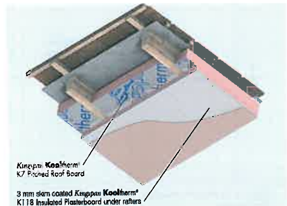
Figure 7 Mechanically fixed to timber rafters with Kingspan Kooltherm ® K7 Pitched Roof Board between rafters
