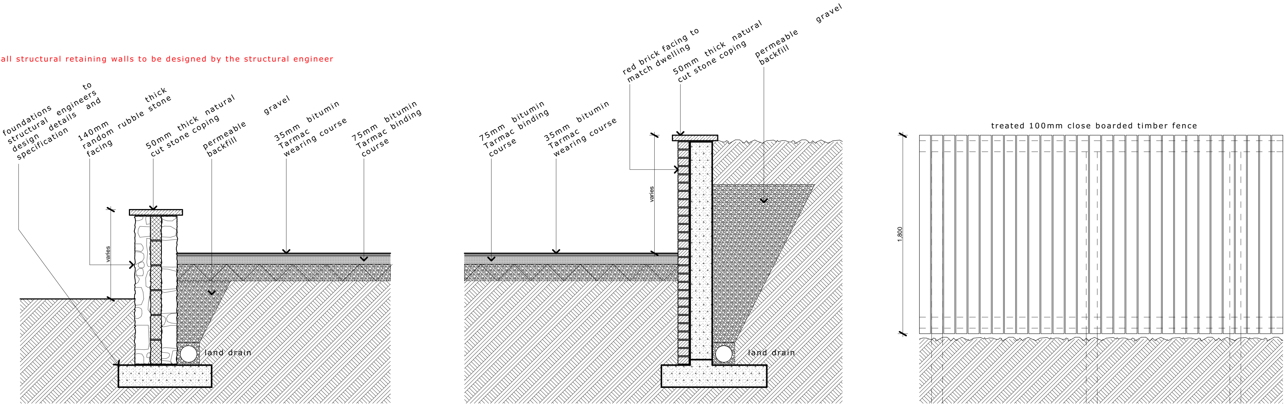
typical boundary wall details 1:20
