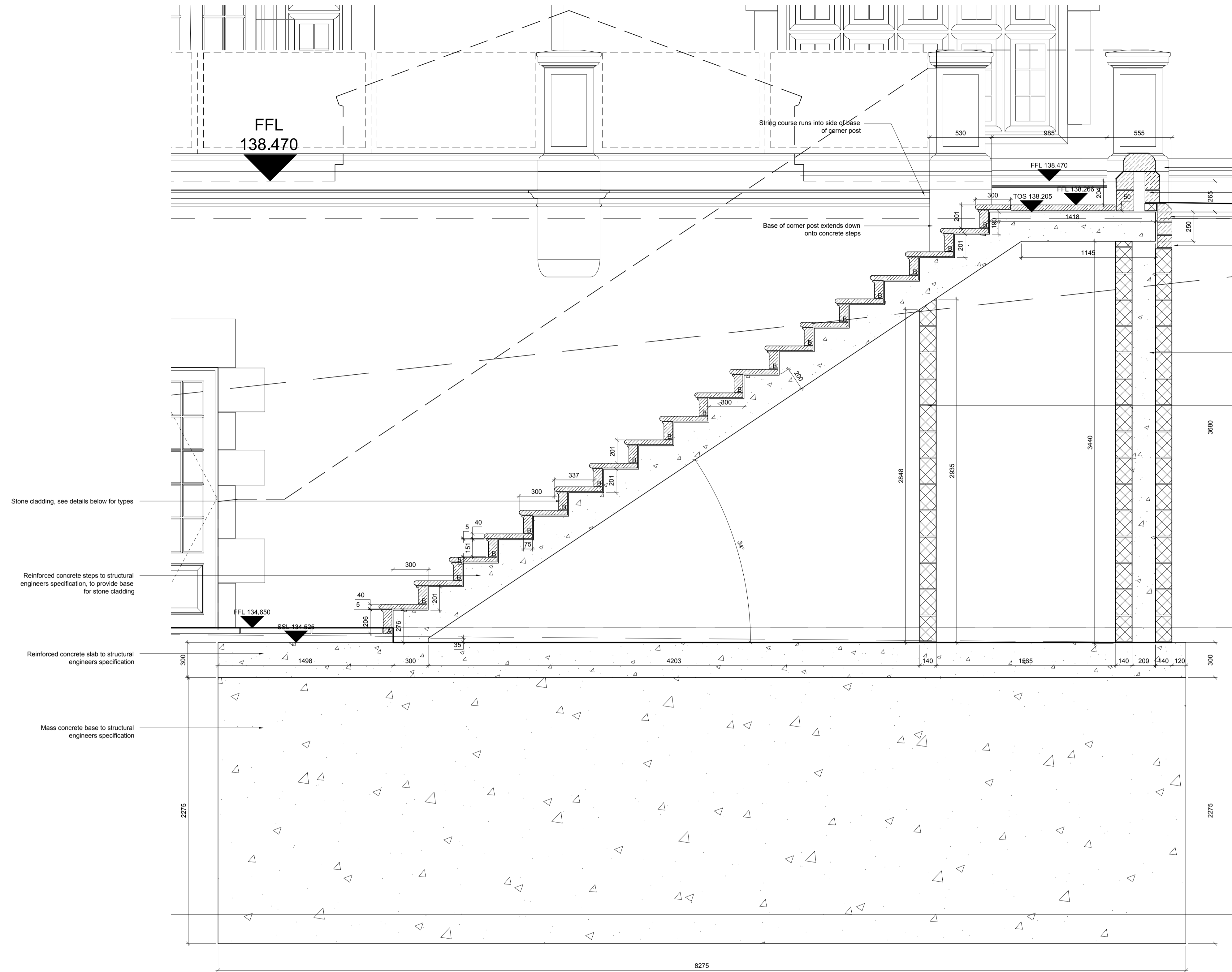
Pool External Stairs Sectional Setting Out 1:20
