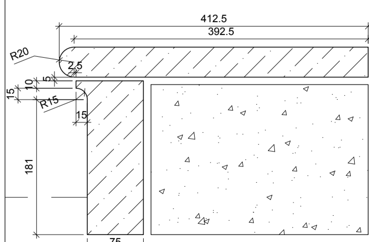
Type A Tread Detail 1:5
