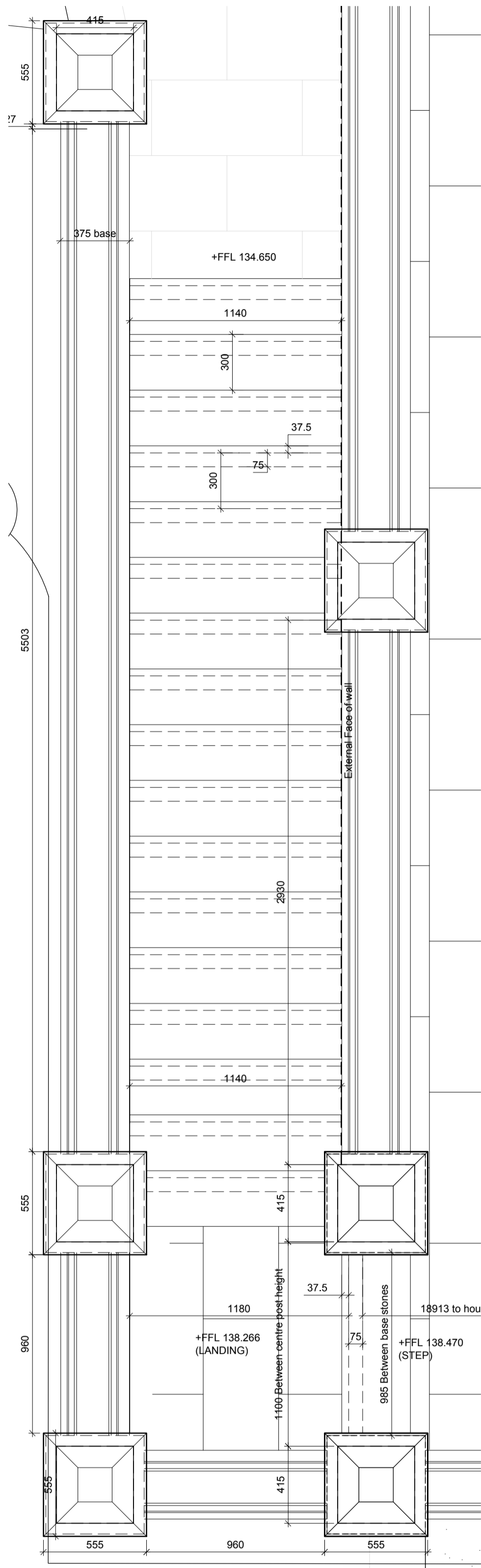
Pool External Stairs Setting Out 1:20
