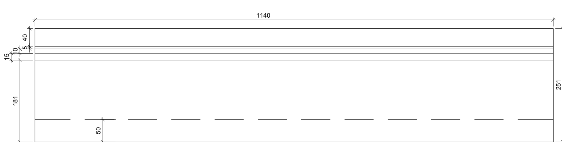
Pool External Stairs Sectional Setting Out 1:20
