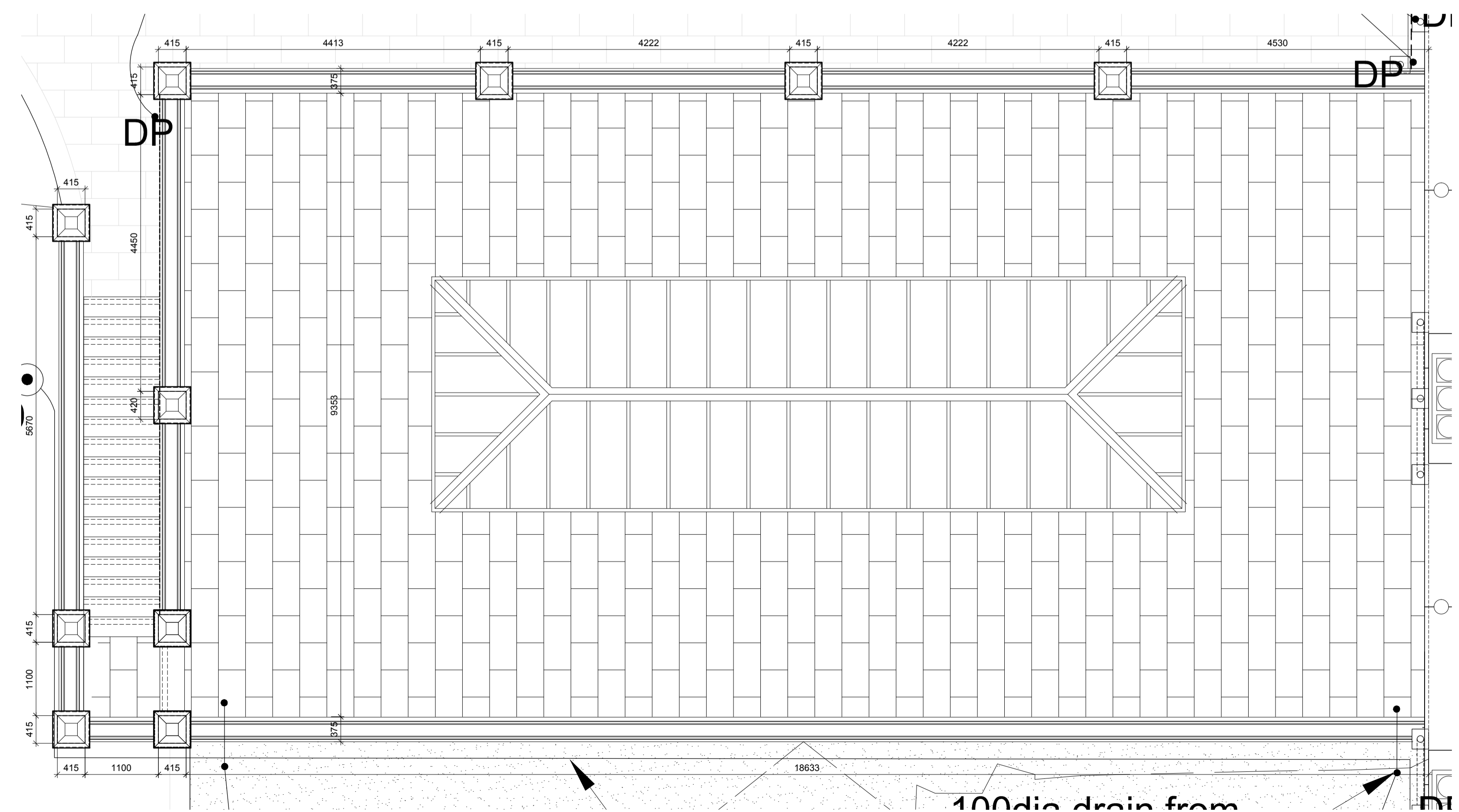
Post Setting Out 1:50
