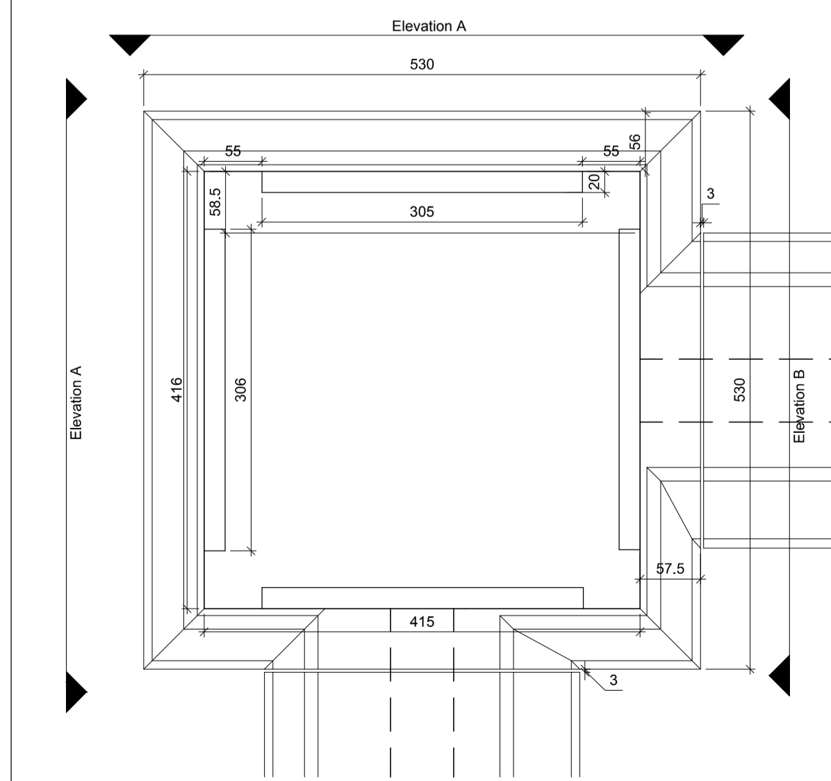
Corner Post Plan Detail 1:5
