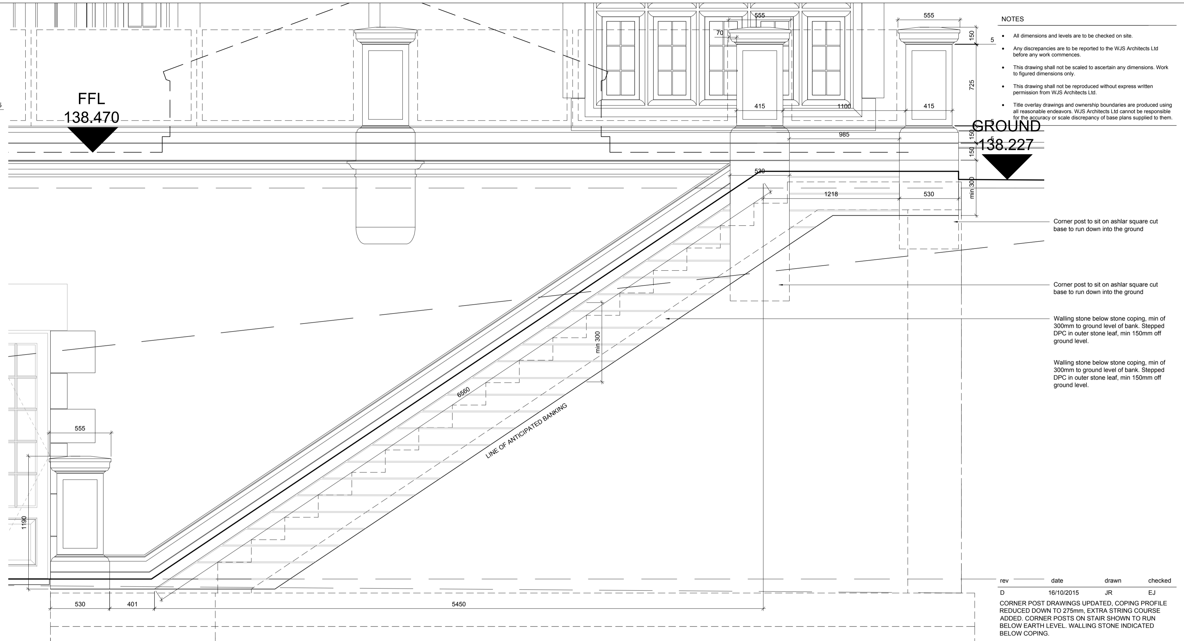
Pool External Stairs Balustrading 1:20
