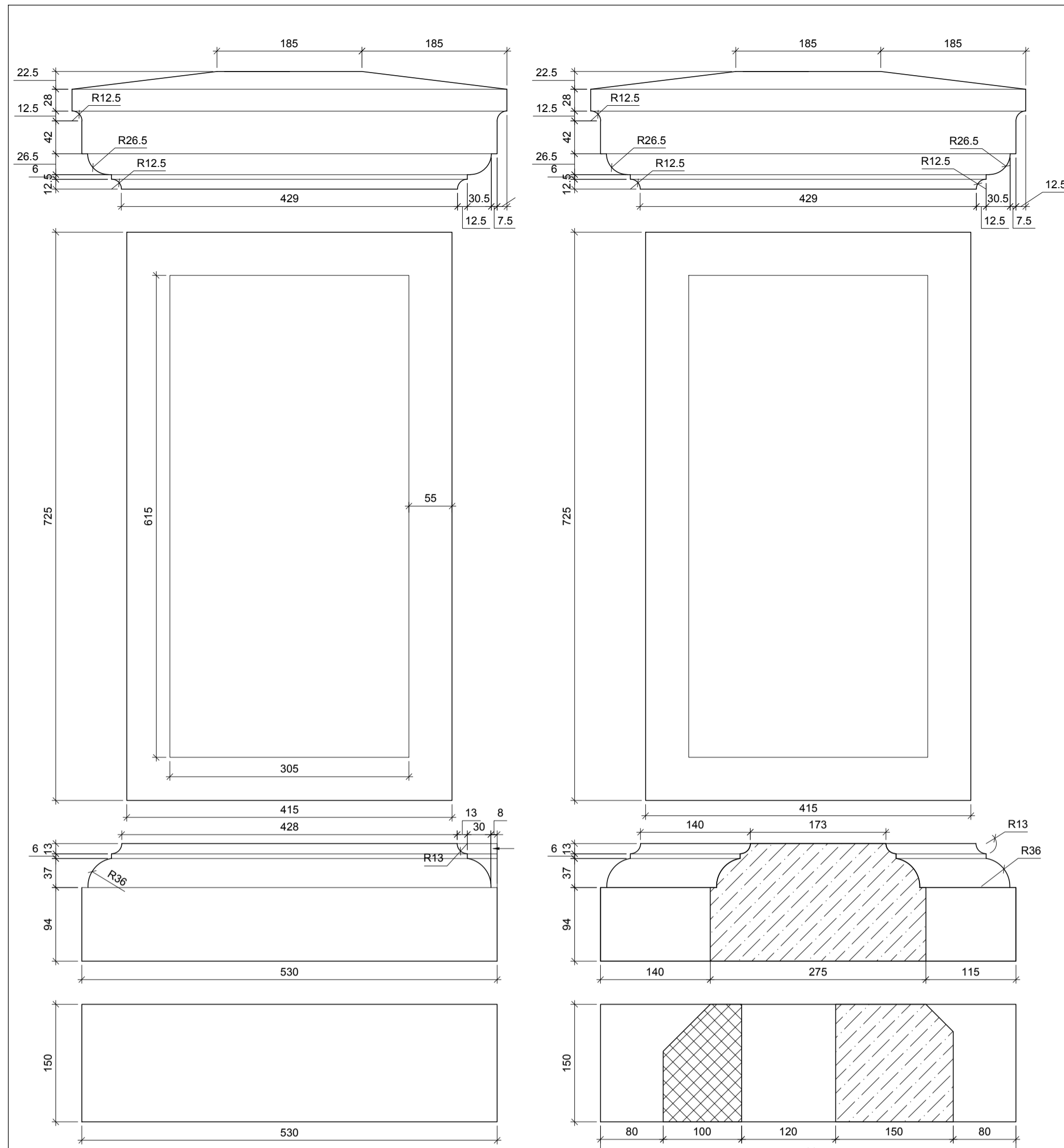
Elevation A Corner Post Elevation Details 1:5
