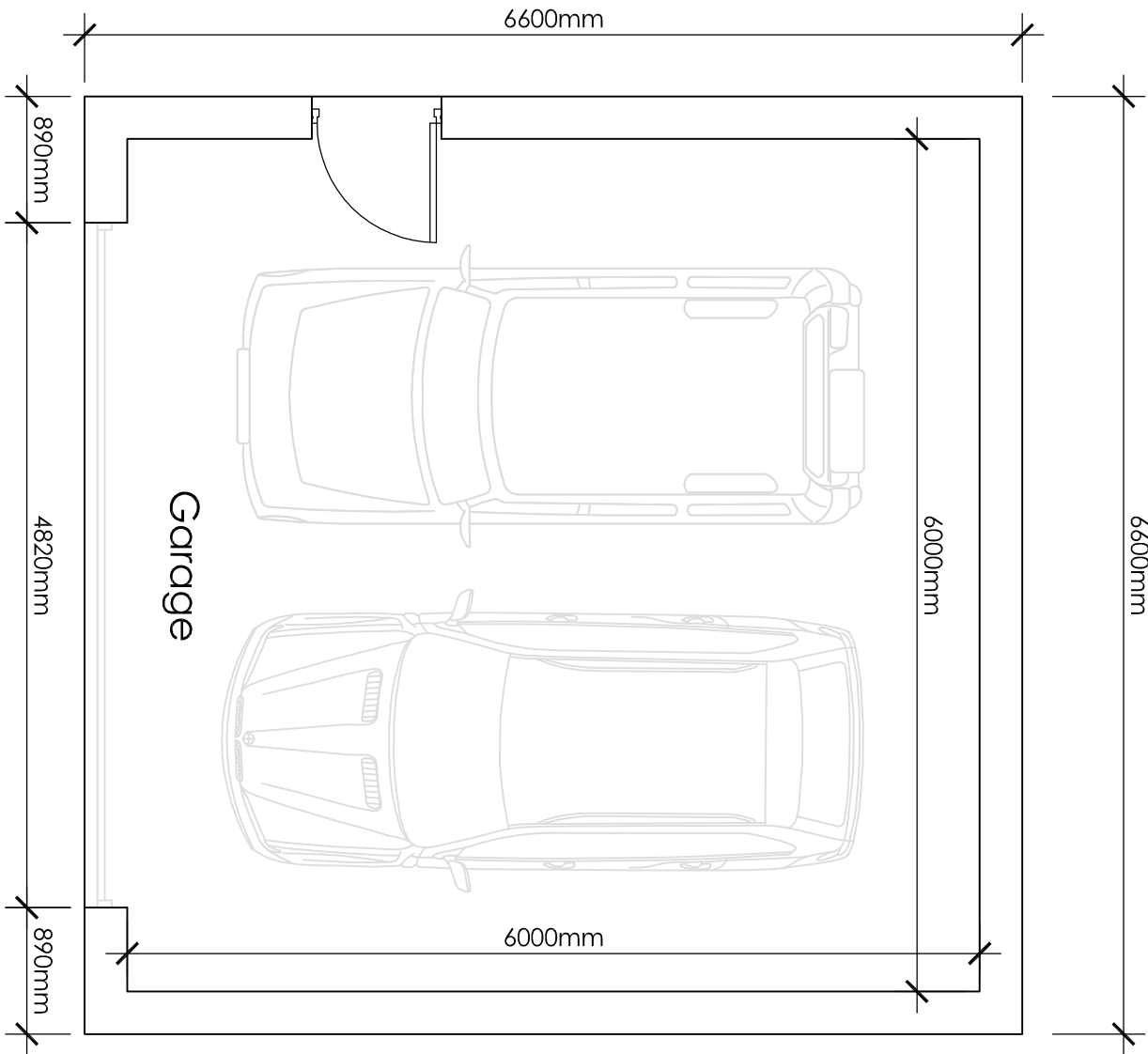
Garage Floor Plan 1:50 Scale
