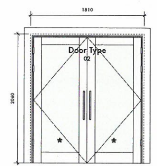
GENERAL ironmongery - 6no hinges - pair 600mm x 19mm dia. straight pull handles - 2no roller catches (to head), fully adjustable glazing - safety glass - clear Dg 7.1 S.O. 1810x2060mm LH hinge Timber architrave to both sides (set within recess)
