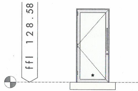
Dg3.1 - g03 utility / bootroom ashlar stone head and cill coursed ashlar stone to jambs clear glass ironmongery - pair 600mm x 19mm dia. straight pull handles - mortice dead lock - double cylinder with thumbturn, and roses - 'stormproof' threshold - draught seals to jamb and head
