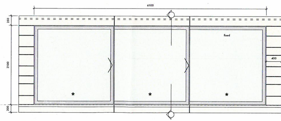
Dg7.2 - g07 kitchen ashlar stone head and cill coursed ashlar stone to jambs clear glass ironmongery by sliding door manufacturer
