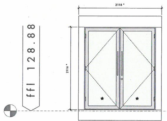
Dg6.2 - g06 lounge existing ashlar stone surround clear glass ironmongery - pair 600mm x 19mm dia. straight pull handles - mortice dead lock - double cylinder with thumbturn, and roses - 'stormproof' threshold - draught seals to jamb and head
