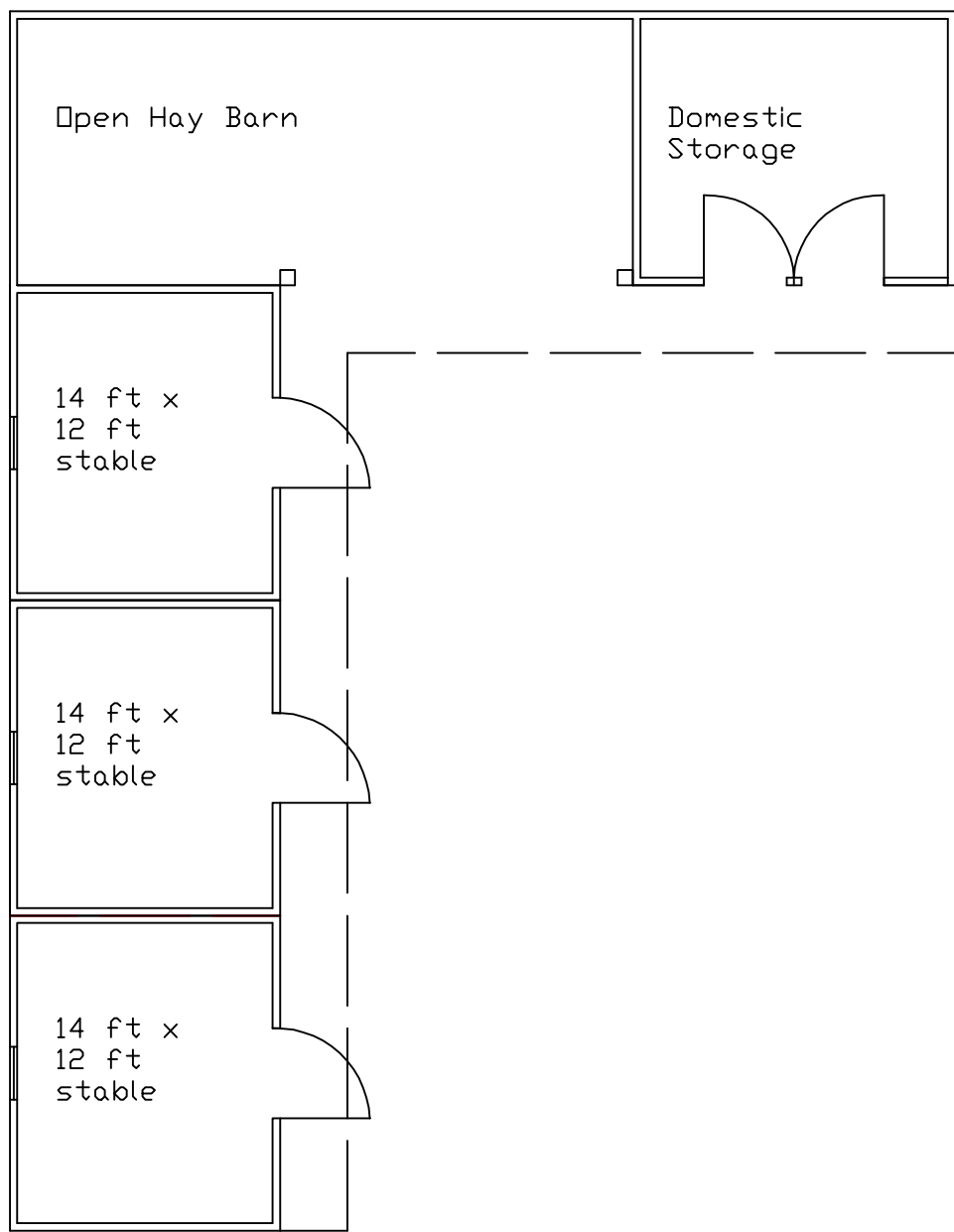
Plan View
