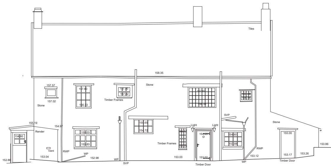
North elevation
