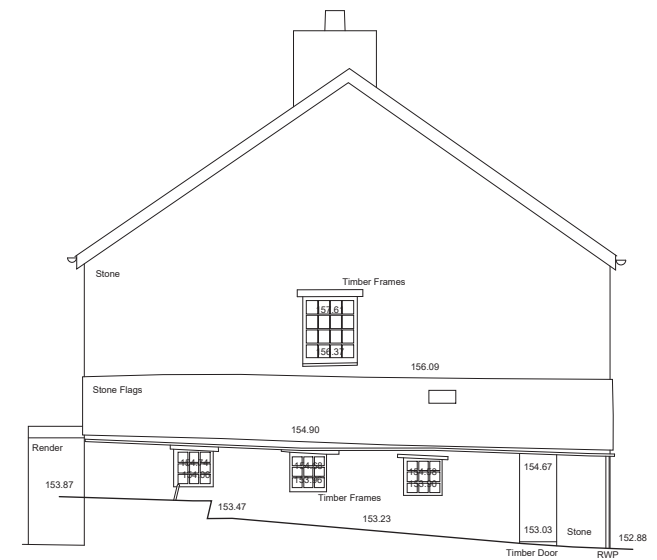
West elevation
