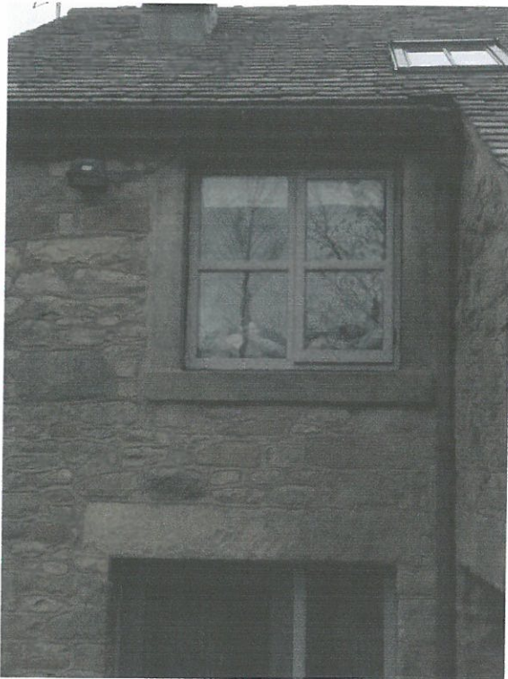
PLATE 1 SUN LOUNGE/NEW OPENING STONE DETAIL TO BE USED AROUND WINDOW REVEALS WITH NATURAL STONE LINTEL VARIOUS SIZES IN HEIGHT ON FACE 150 MM, 200 MM 300 MM .APPROX 150MM DEPTH.RANDOM STONE WALLING VARIOUS SIZES TO BE BUILT UP TO MATCH APPEARANCE.
