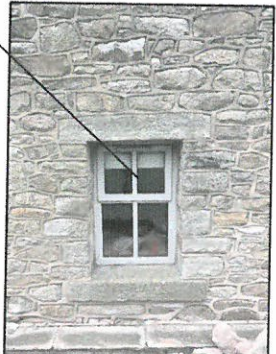
PLATE 6 Existing sandstone details lintel head and sill with weathered sill with dressed stone square stone to reveals
