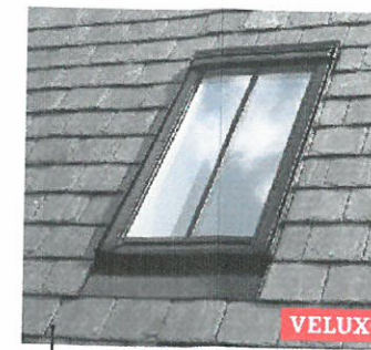
PLATE 5 Detail of Velux Conservation roof light the type to be installed on site to match the existing
