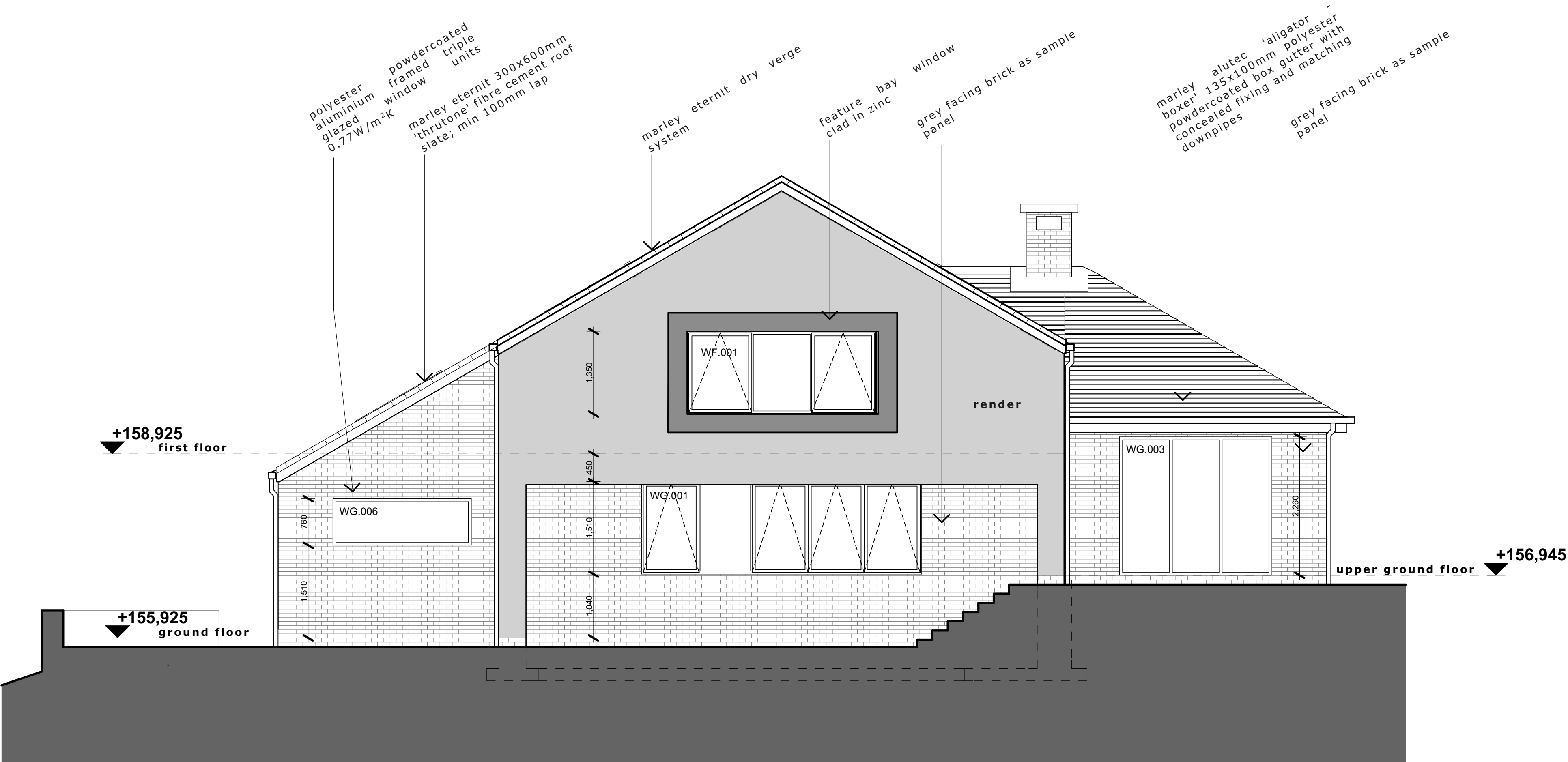
south 1:50
