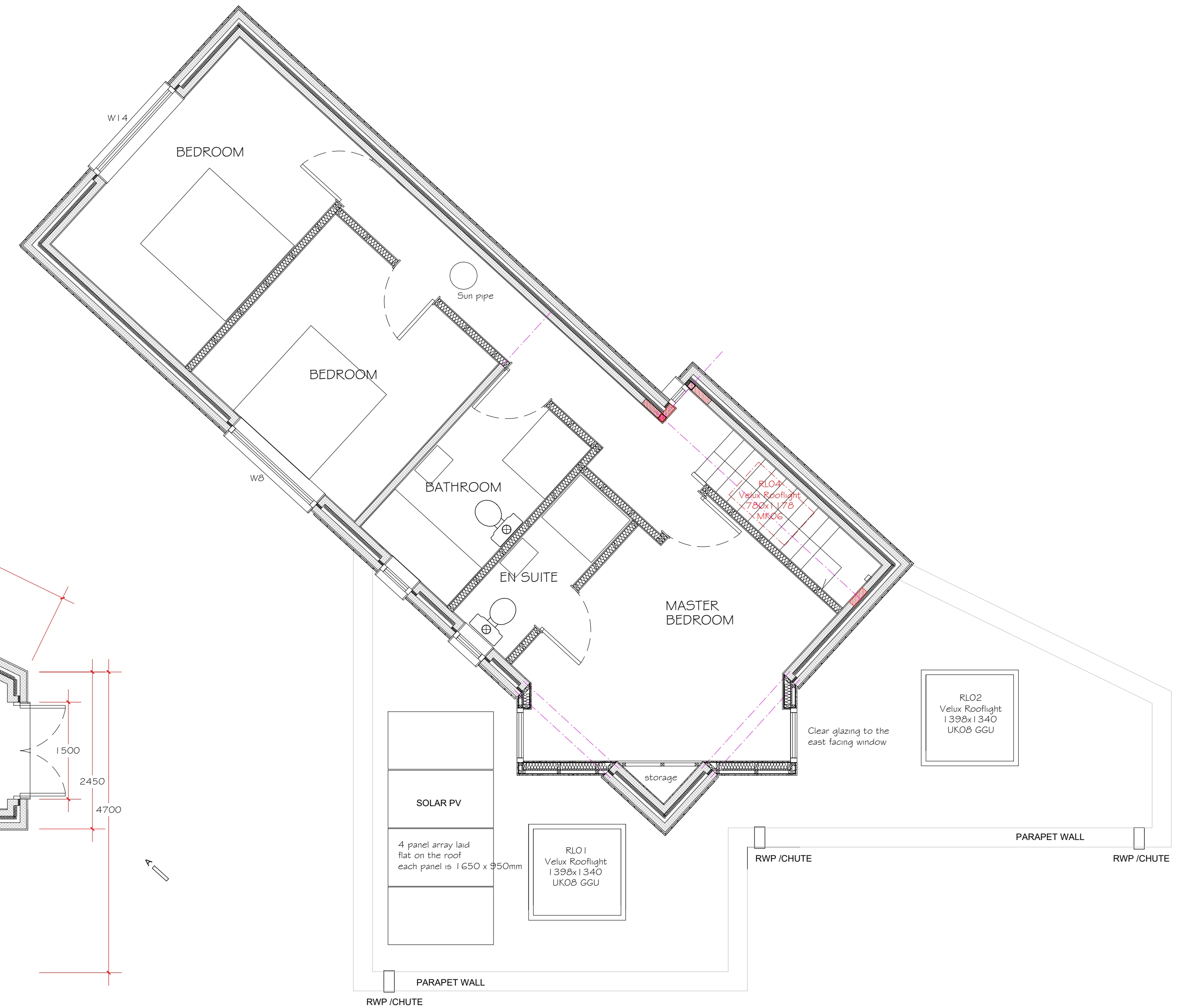
PROPOSED FIRST FLOOR WITH FLAT ROOF PLAN
