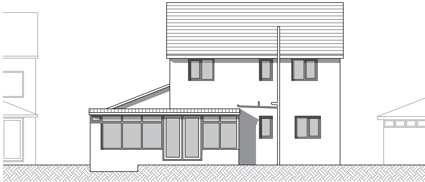
EXISTING SOUTH-EAST ELEVATION
