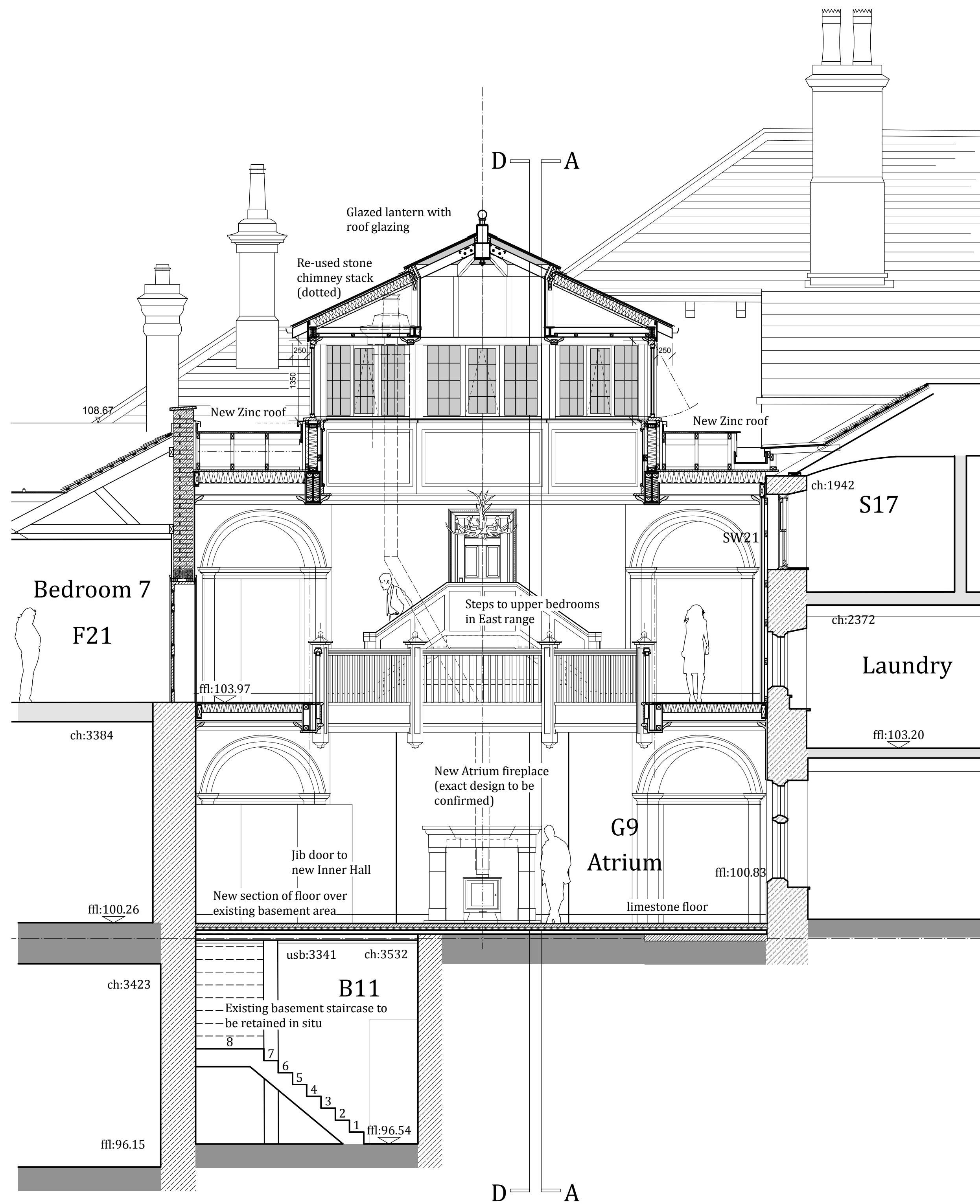
East Facing Section B-B
