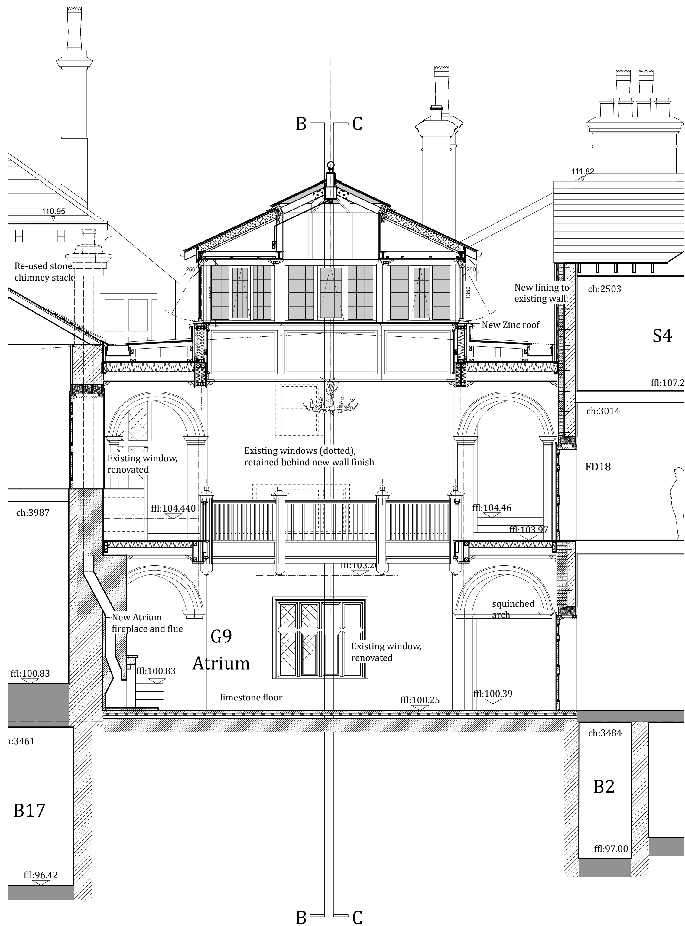
South Facing Section A-A
