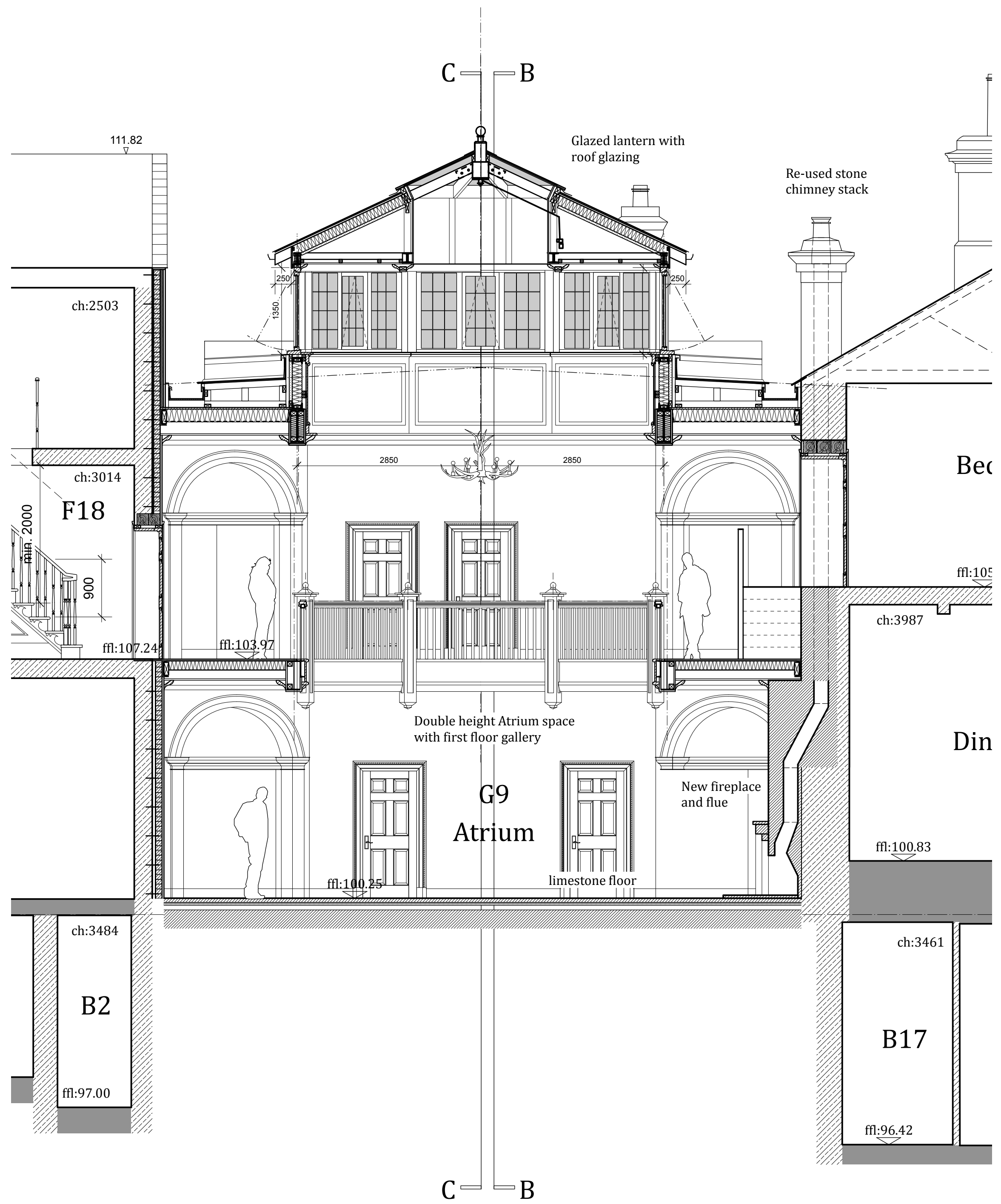
North Facing Elevation D-D
