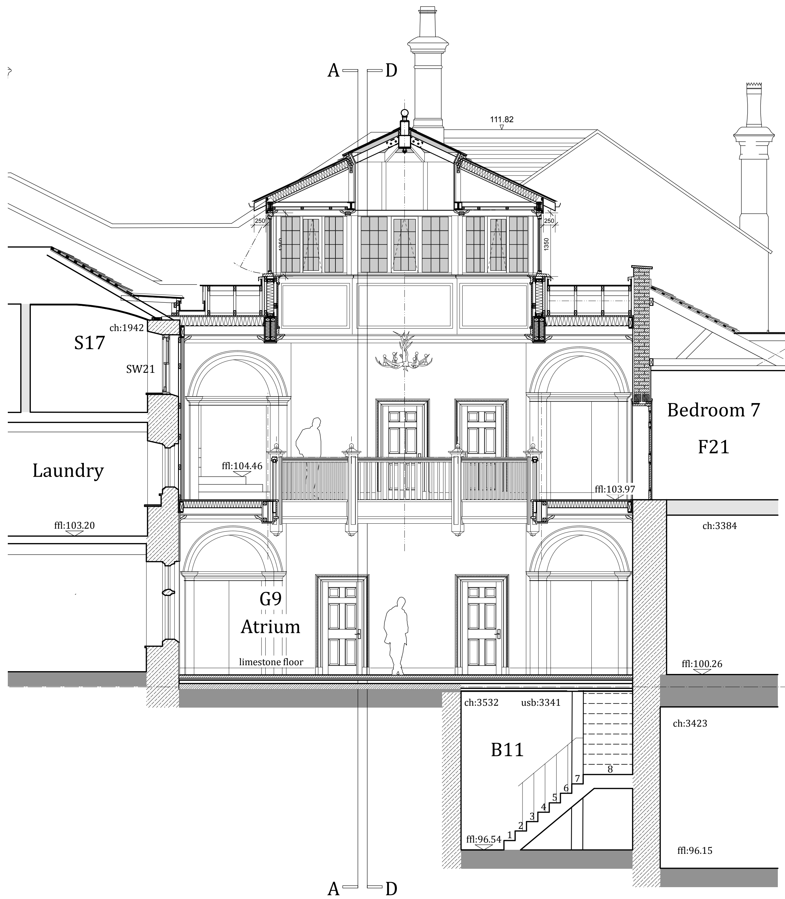
West Facing Section C-C
