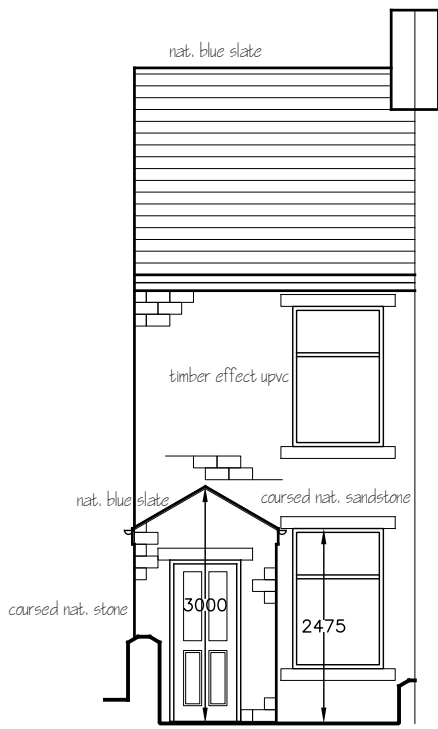
Front Elevation
