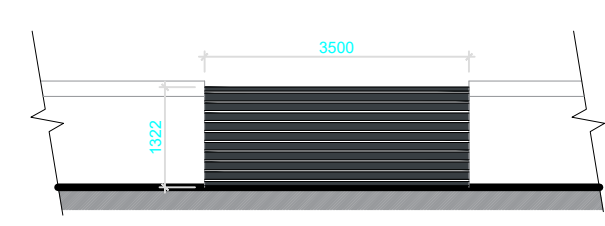
Proposed Elevation (Gate Closed)
