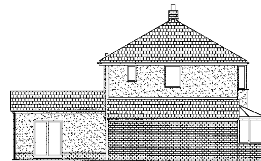
Existing End Elevation
