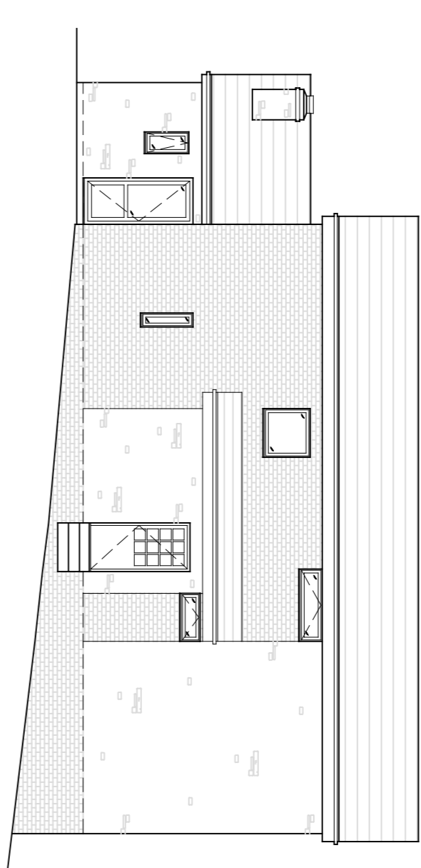
Side Elevation (Facing North)
