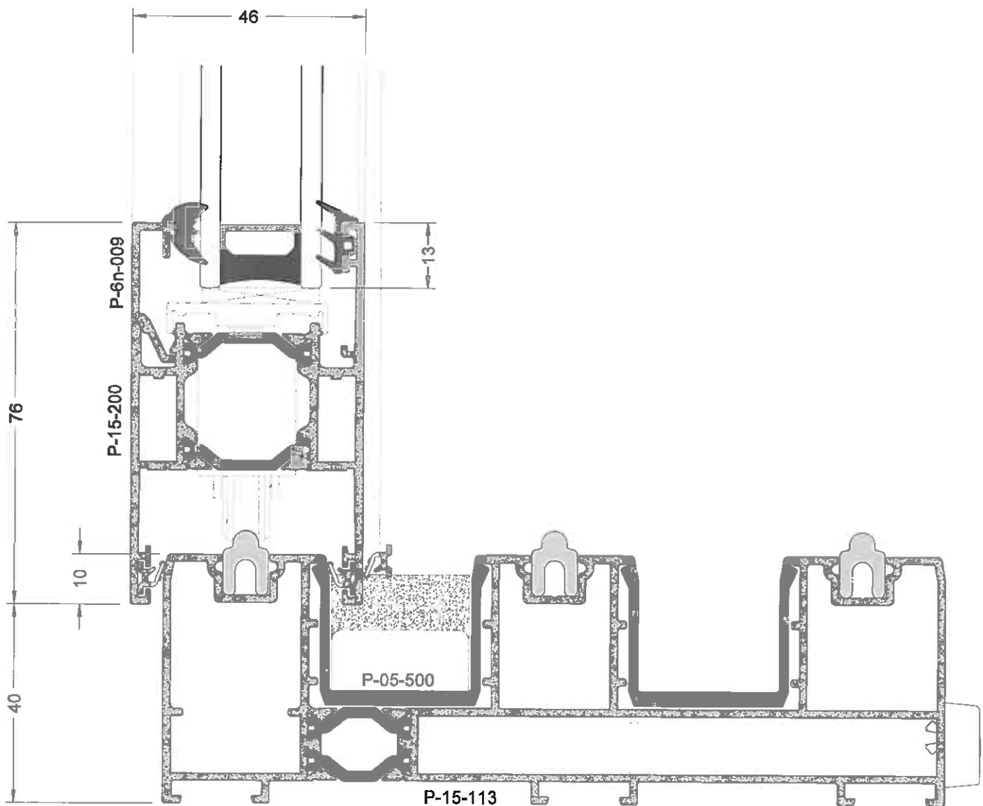
Inline Slide
