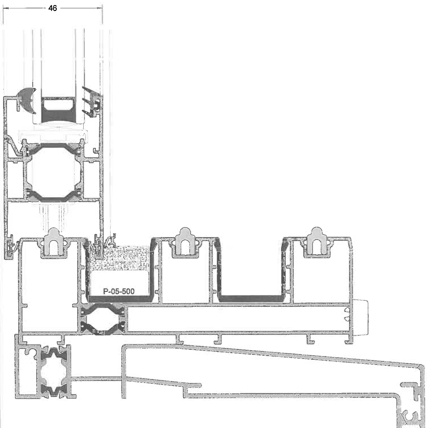
Inline Slide
