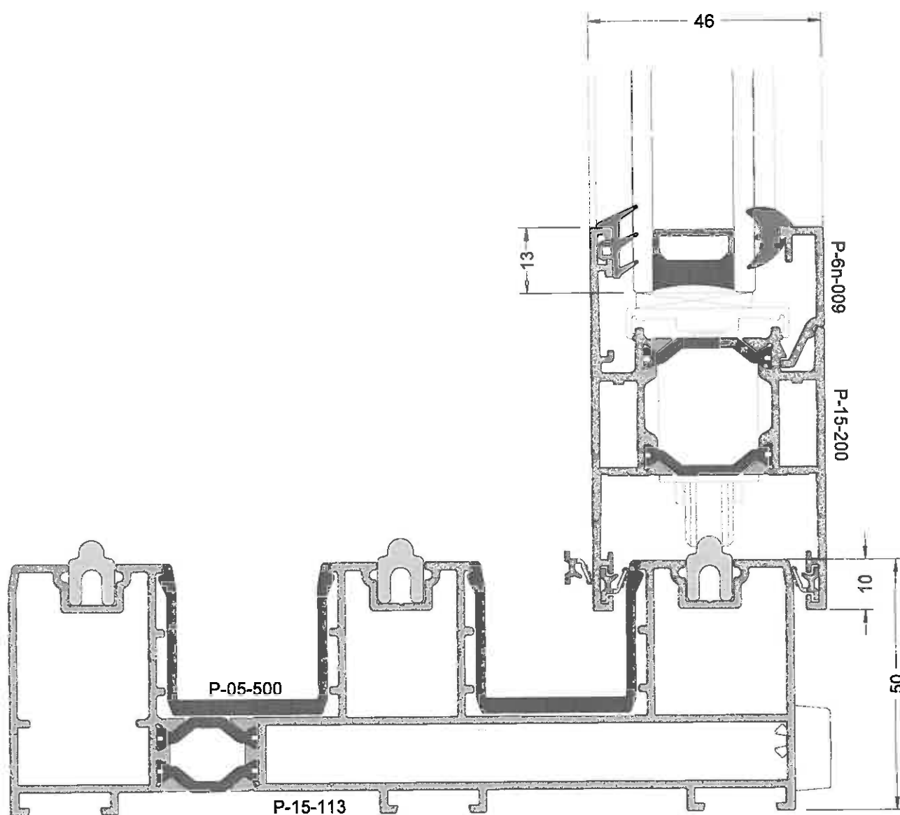
Inline Slide
