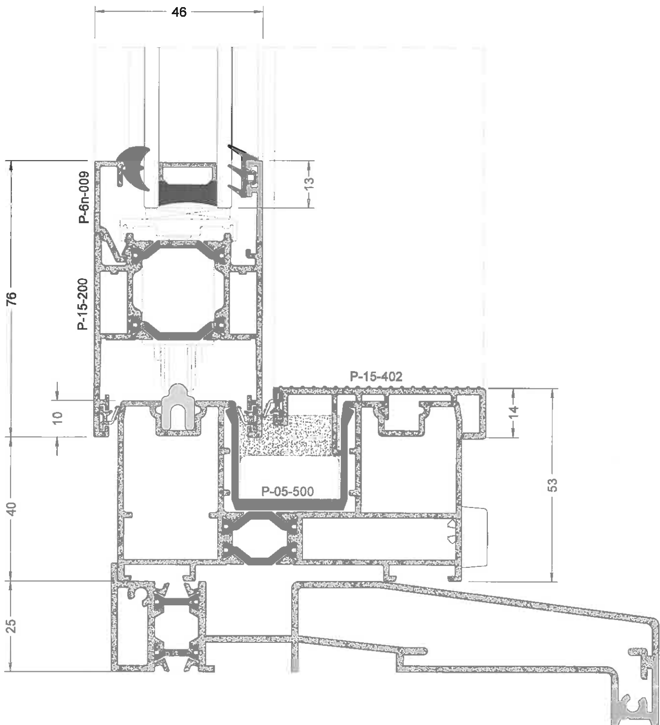
Inline Slide
