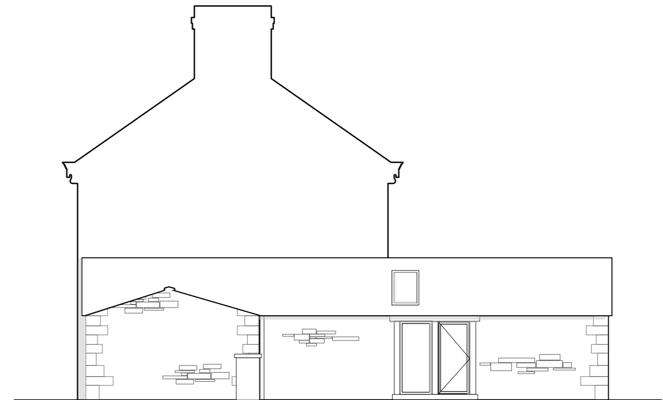
2 Front Elevation
