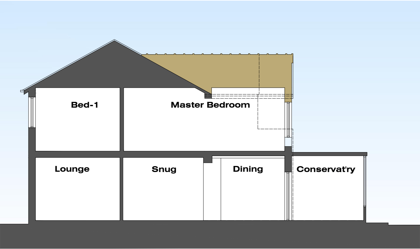
Side (South-East) Sectional Elevation
