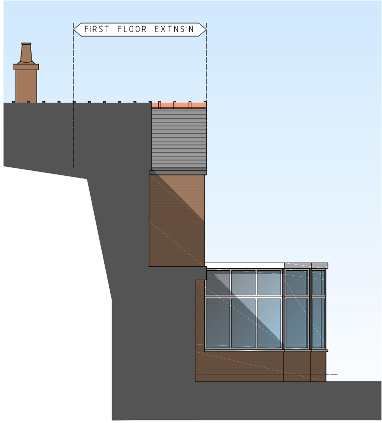
Side (South-East) Elevation
