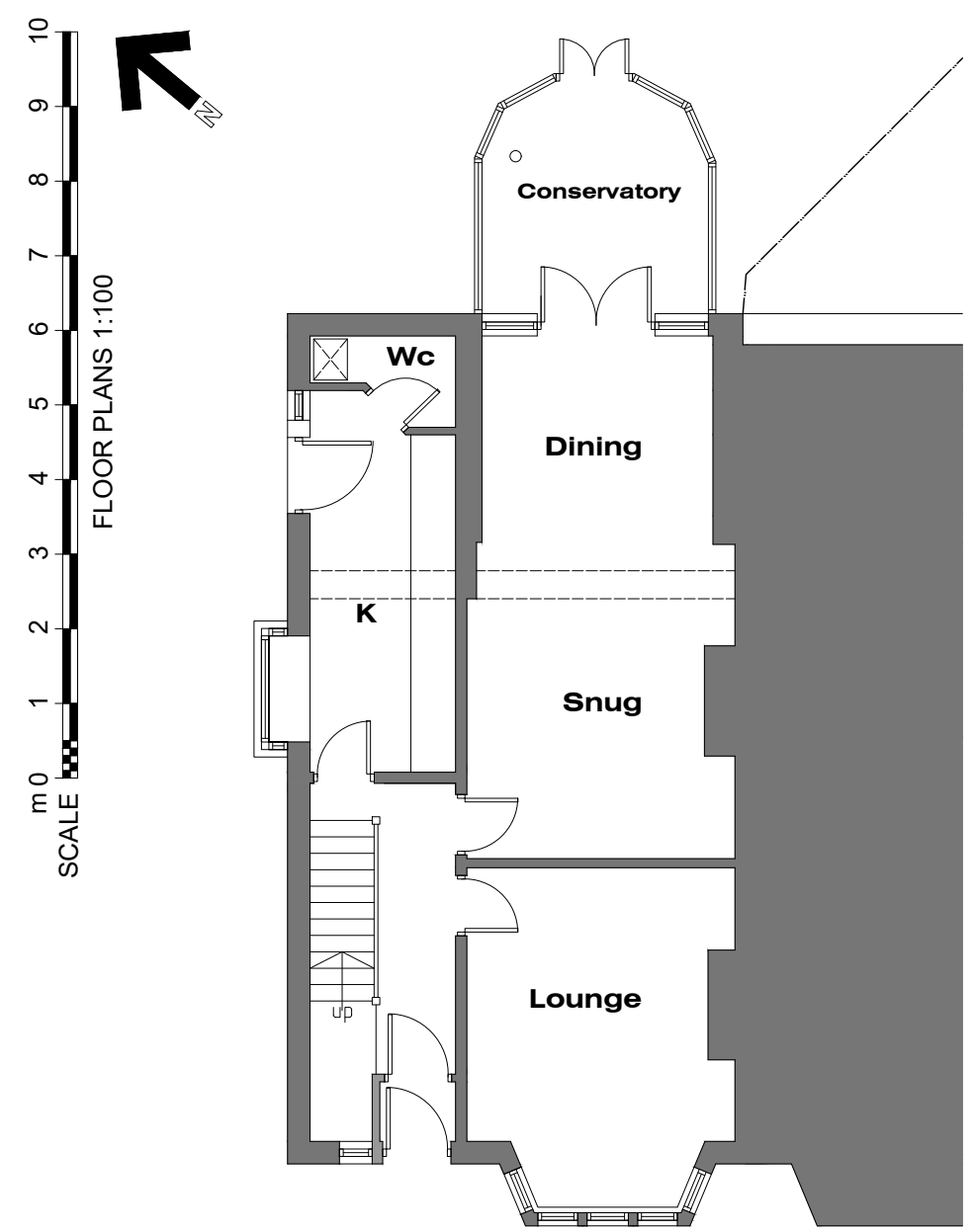
GROUND FLOOR
