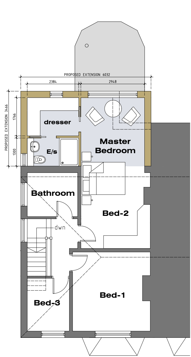
FIRST FLOOR SK-1
