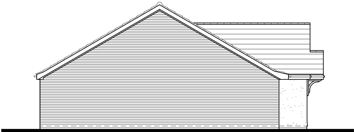
Side elevation
