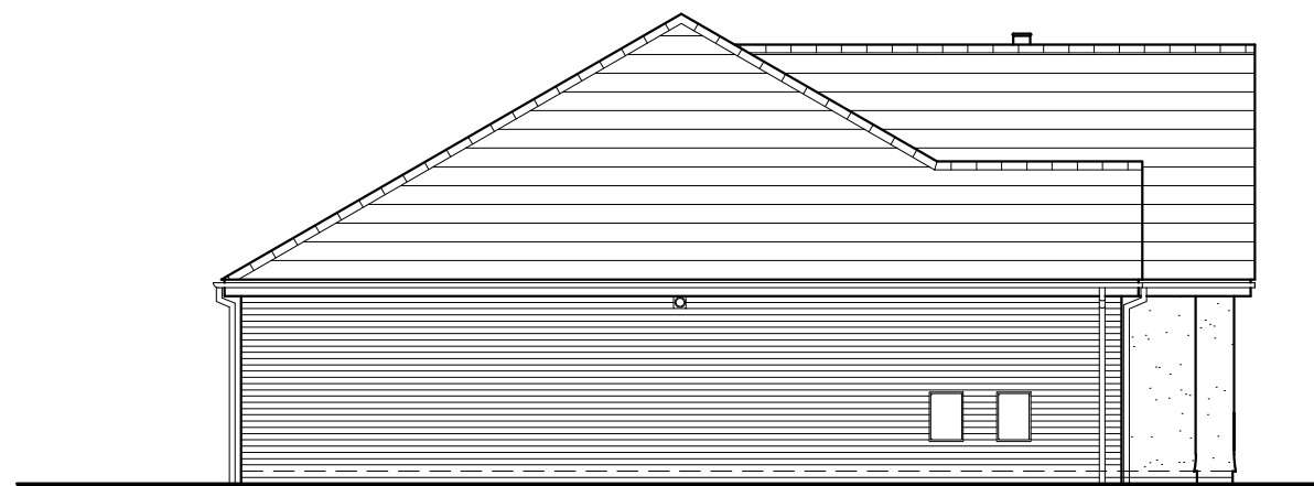
Side elevation
