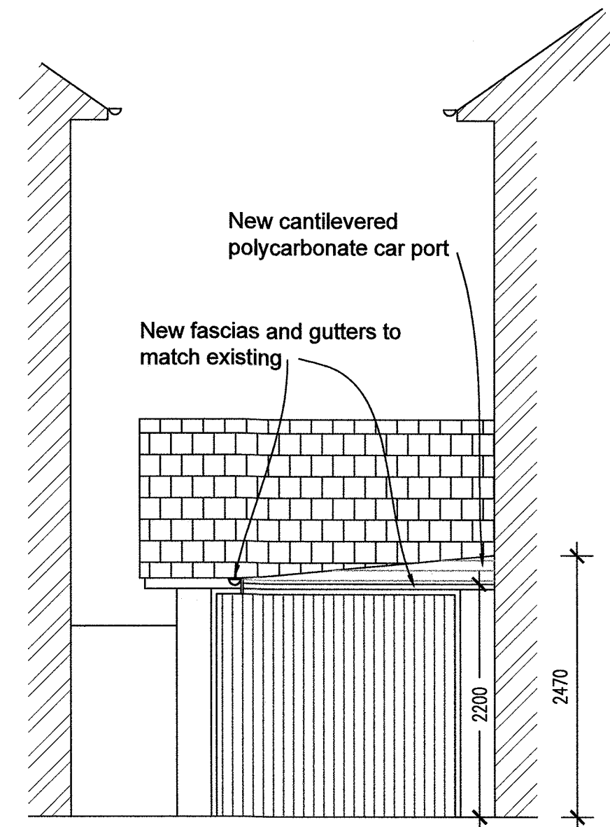
Proposed Elevation
