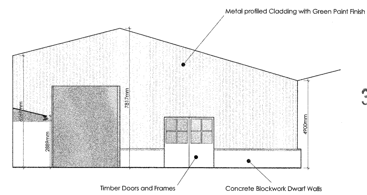
South West Facing Elevation Scale 1:100
