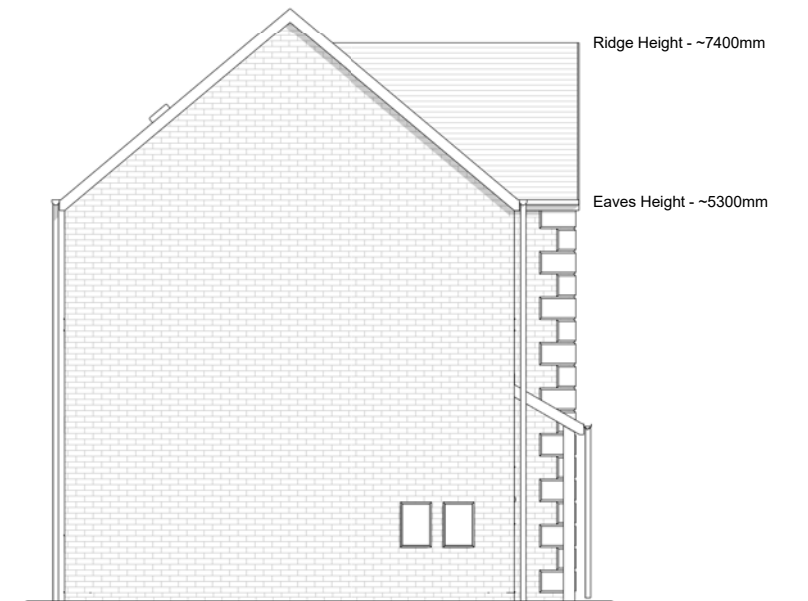
Left Elevation 1 : 100
