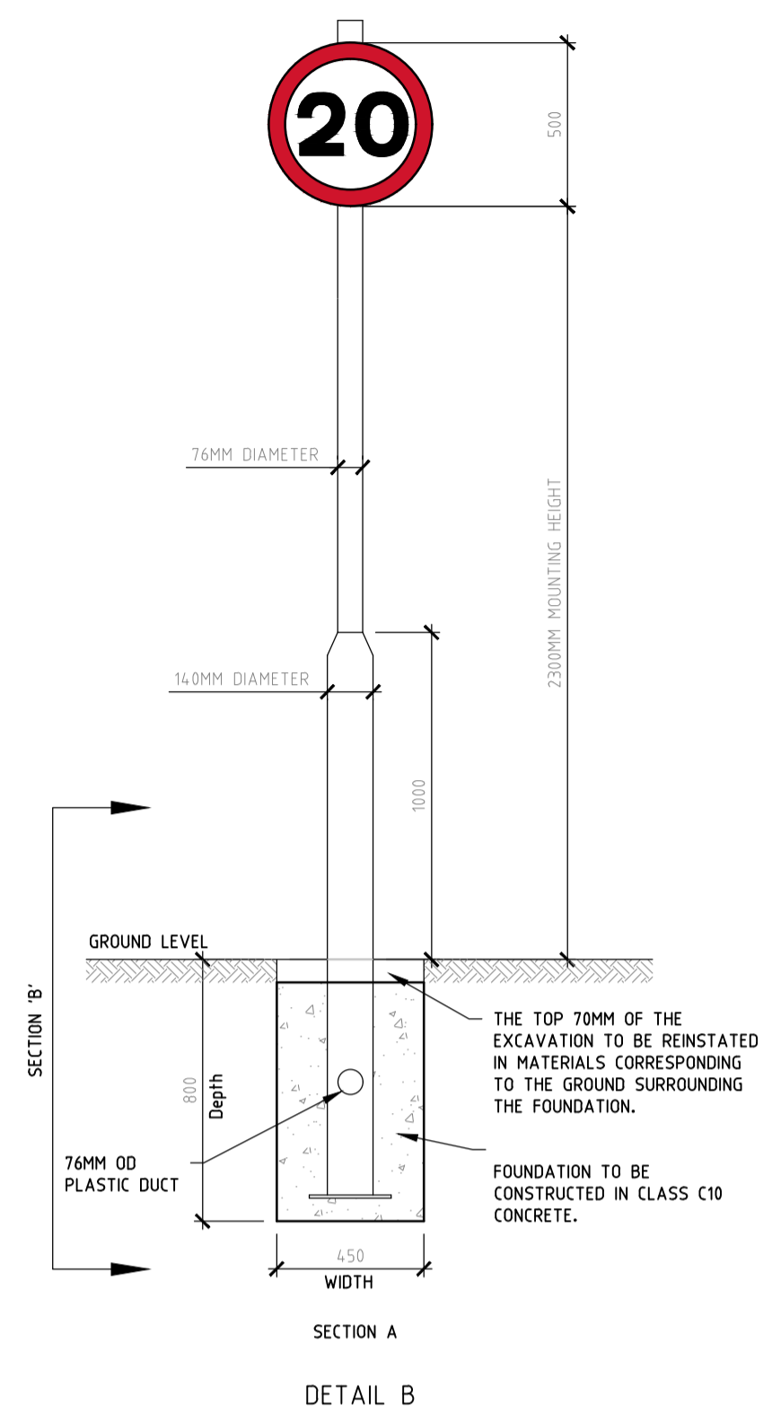
DETAIL B
