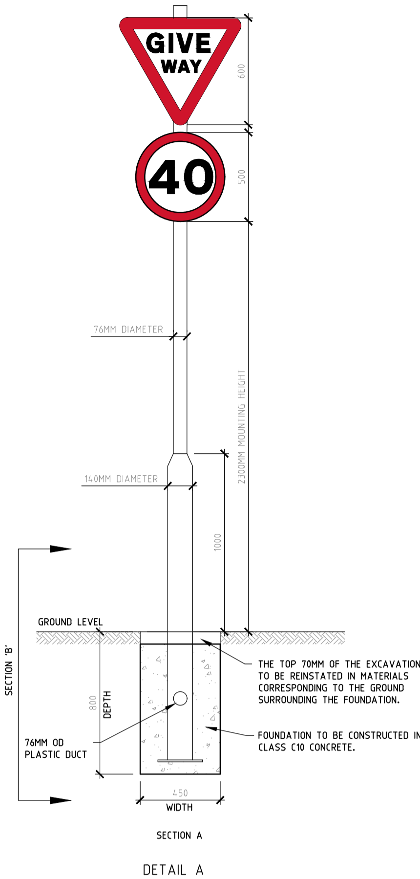
DETAIL A
