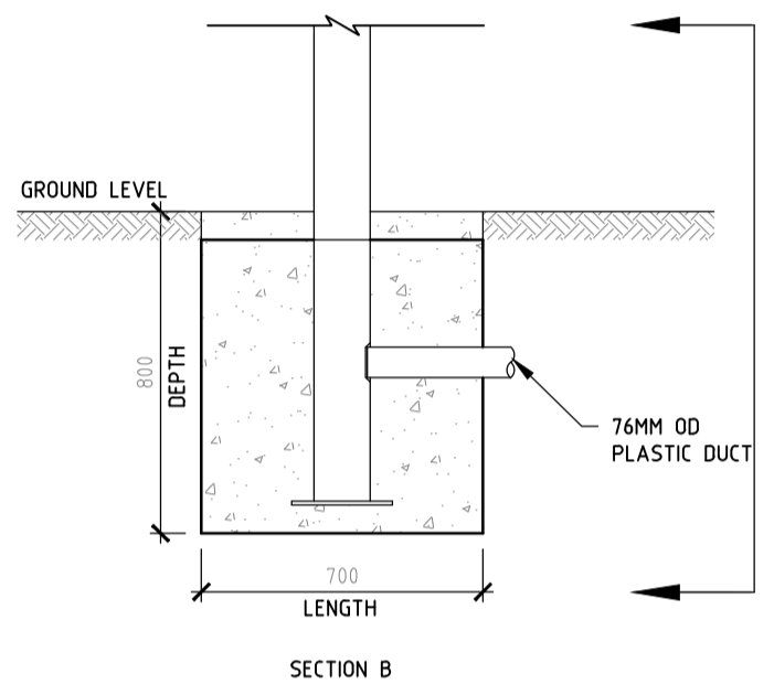
SECTION B
