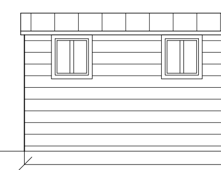
NORTHERN ELEVATION
