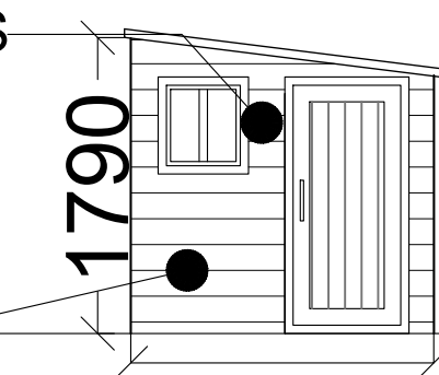
EASTERN ELEVATION
