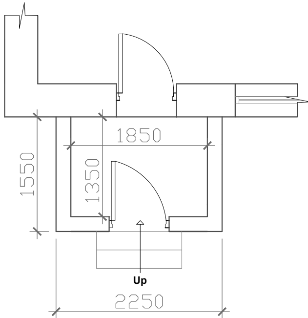
Floor Plan 1:50 Scale
