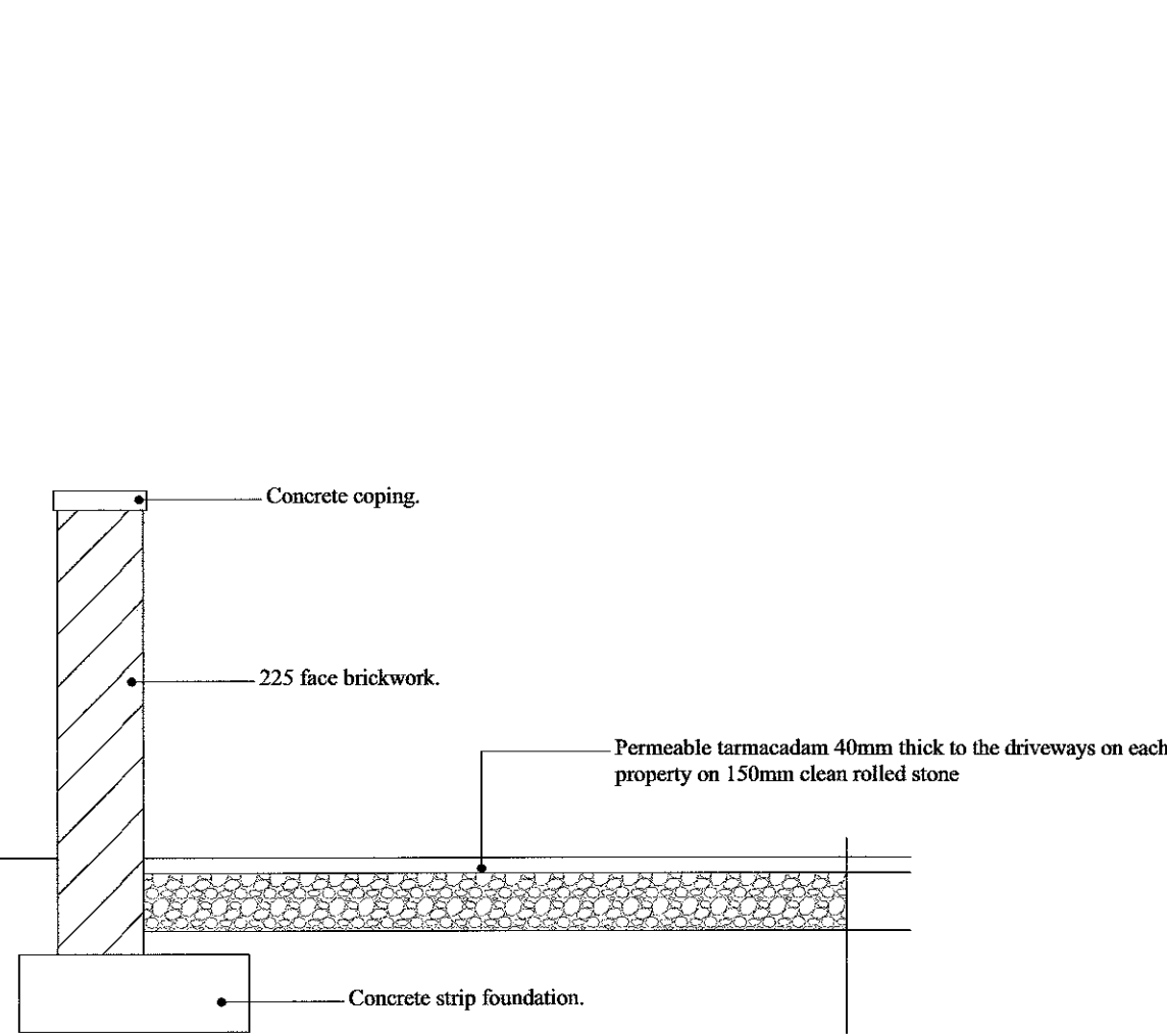
Boundary Wall Detail B.
