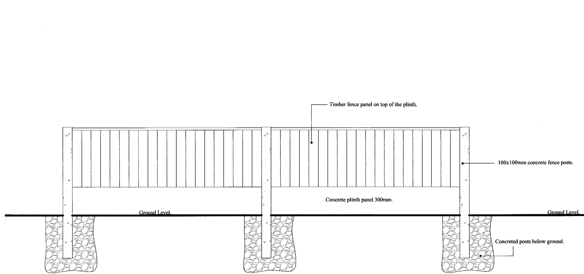
Party Fence Detail A.
