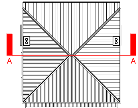
Roof Plan (1:200 scale)
