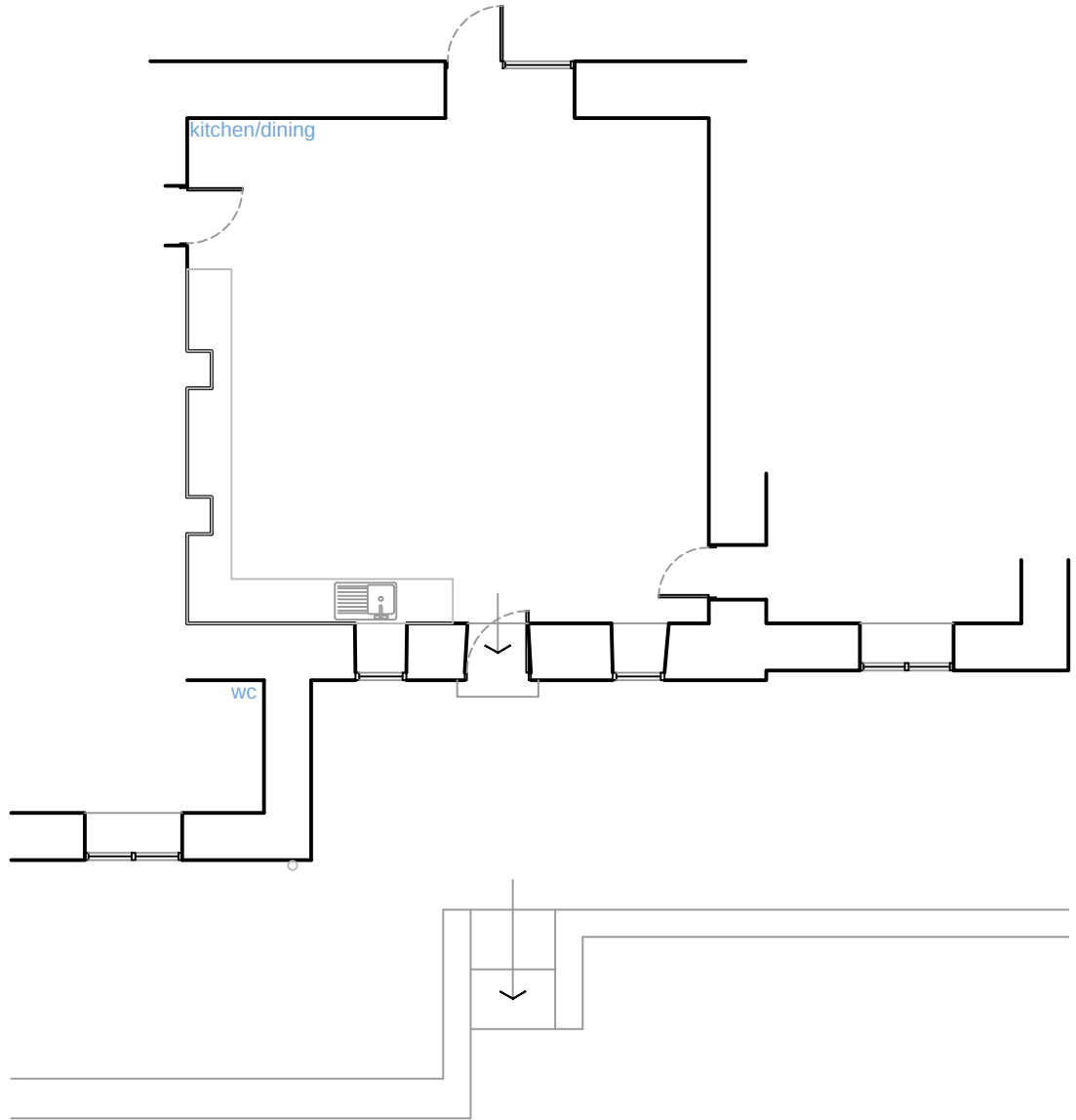
GROUND FLOOR PLAN AS EXISTING
