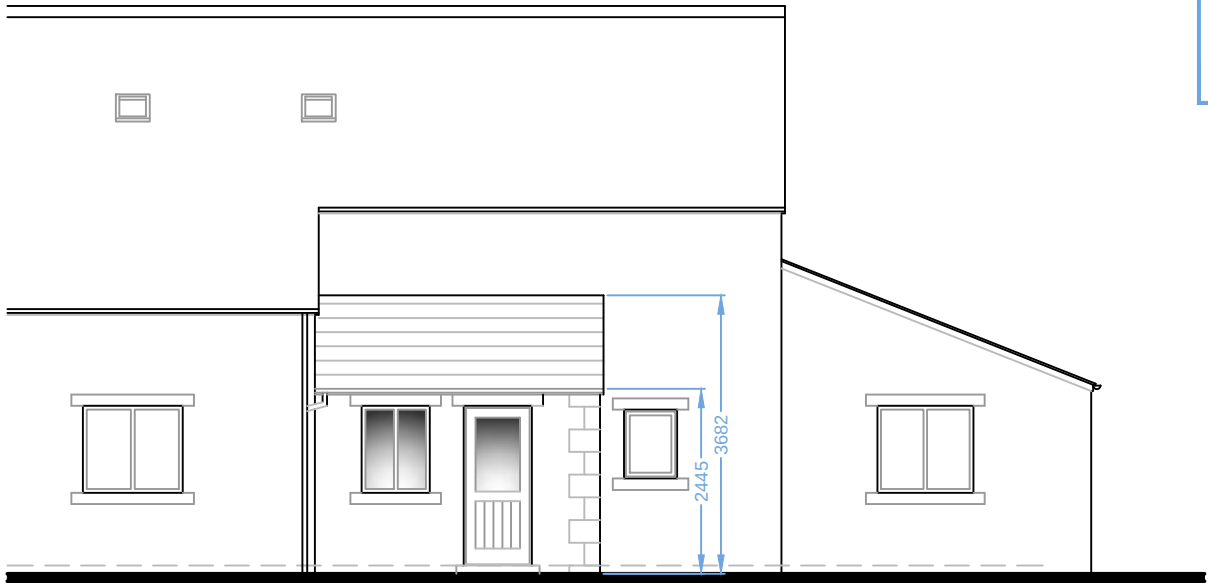
PART FRONT ELEVATION AS PROPOSED
