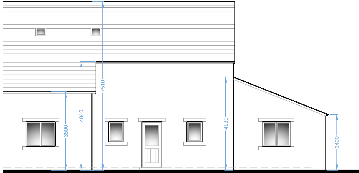
PART FRONT ELEVATION AS EXISTING
