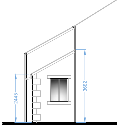
PART SIDE ELEVATION AS PROPOSED
