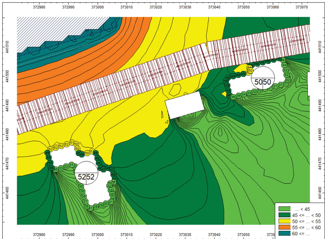
Figure 7: Predicted AGP Noise Emission (1.5 metres above the ground).
