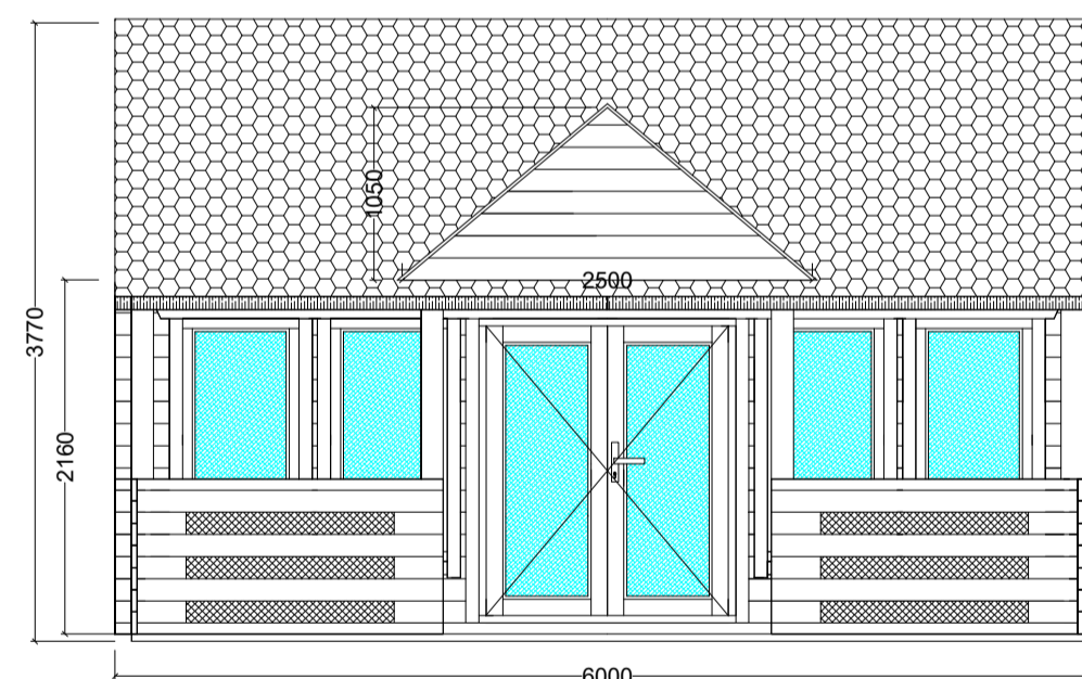
Wooden Storage / Site Office - Front View
