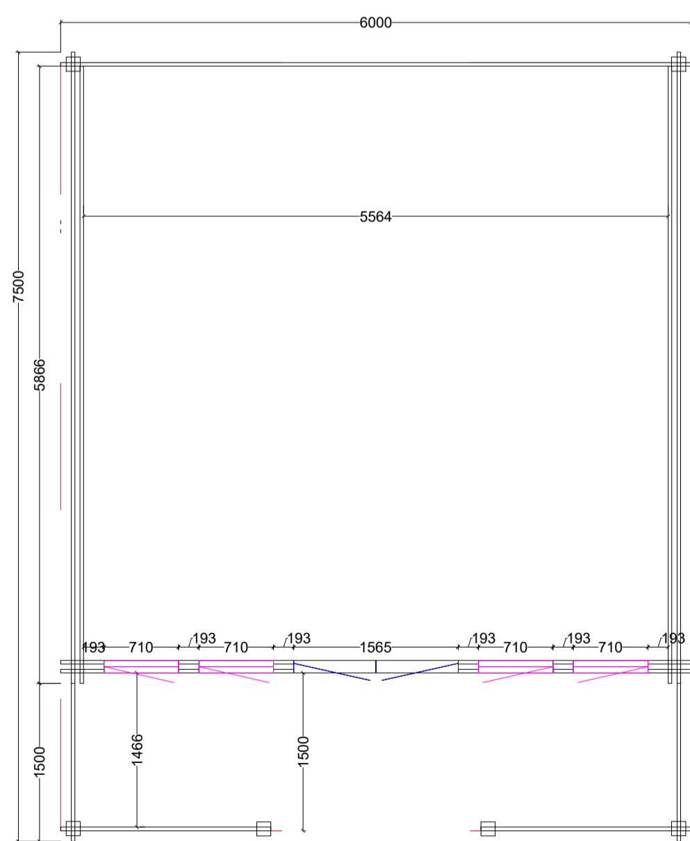
Wooden Storage / Site Office - Plan View
