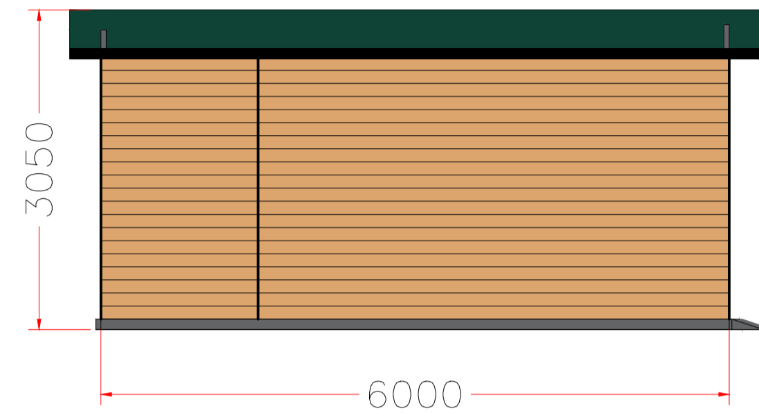
Maintenance equipment store - Side View
