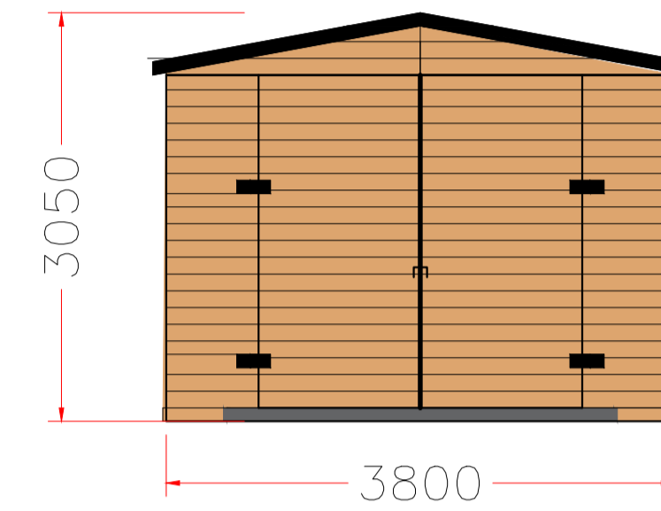
Maintenance equipment store - Front View
