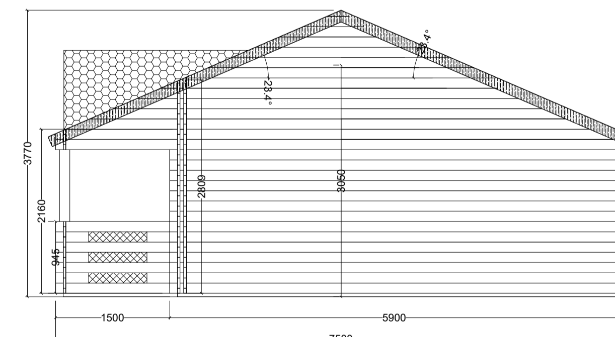
Wooden Storage / Site Office - Side View
