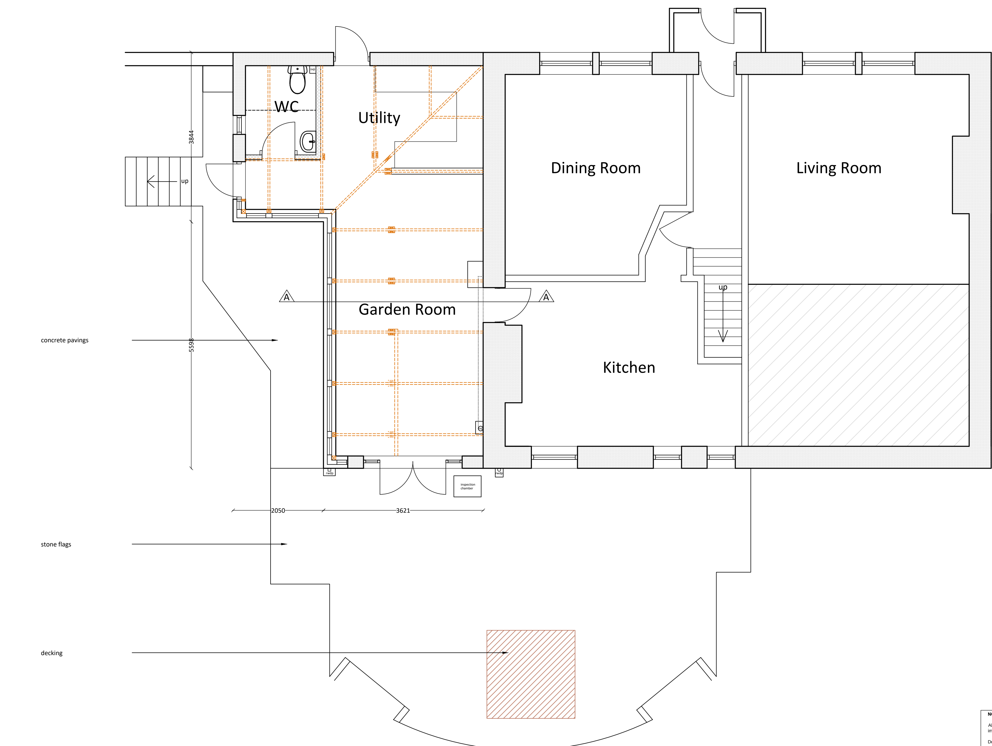
EXISTING GROUND FLOOR PLAN 1: 50 @ A1
