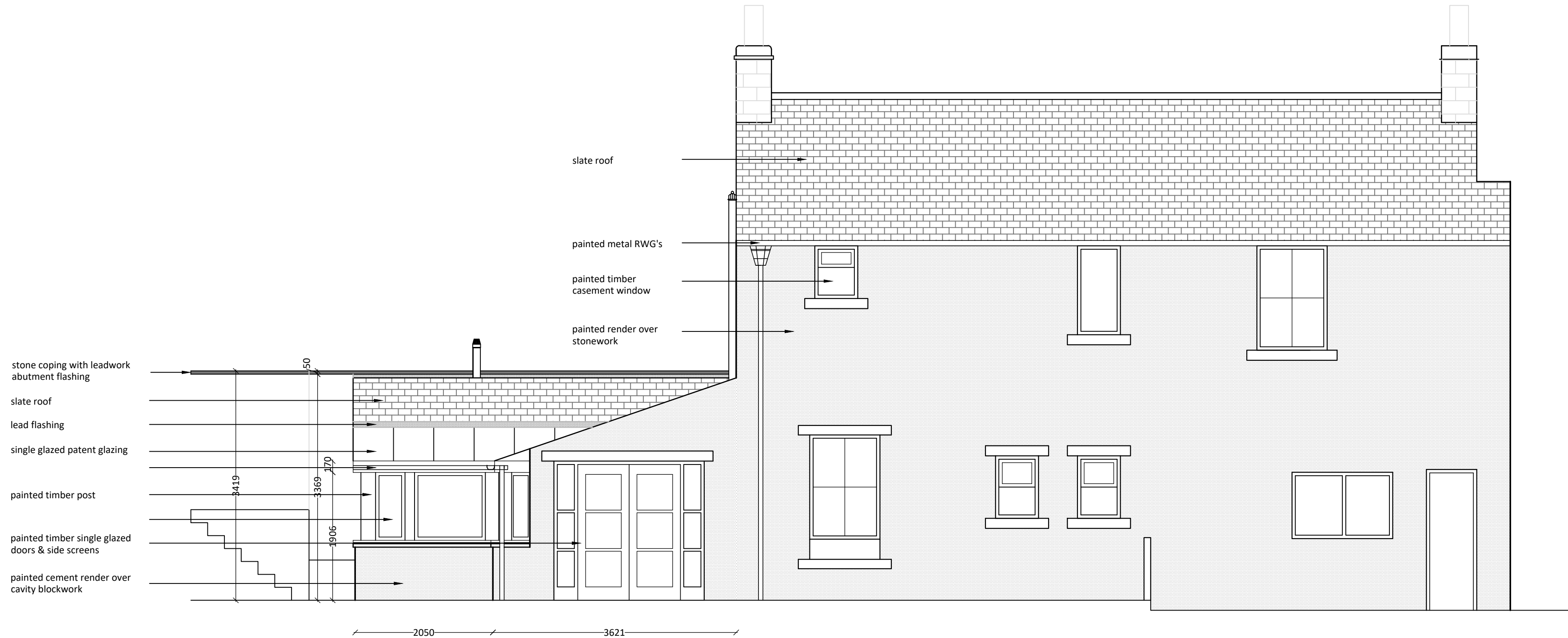
EXISTING REAR ELEVATION 1: 50 @ A1
