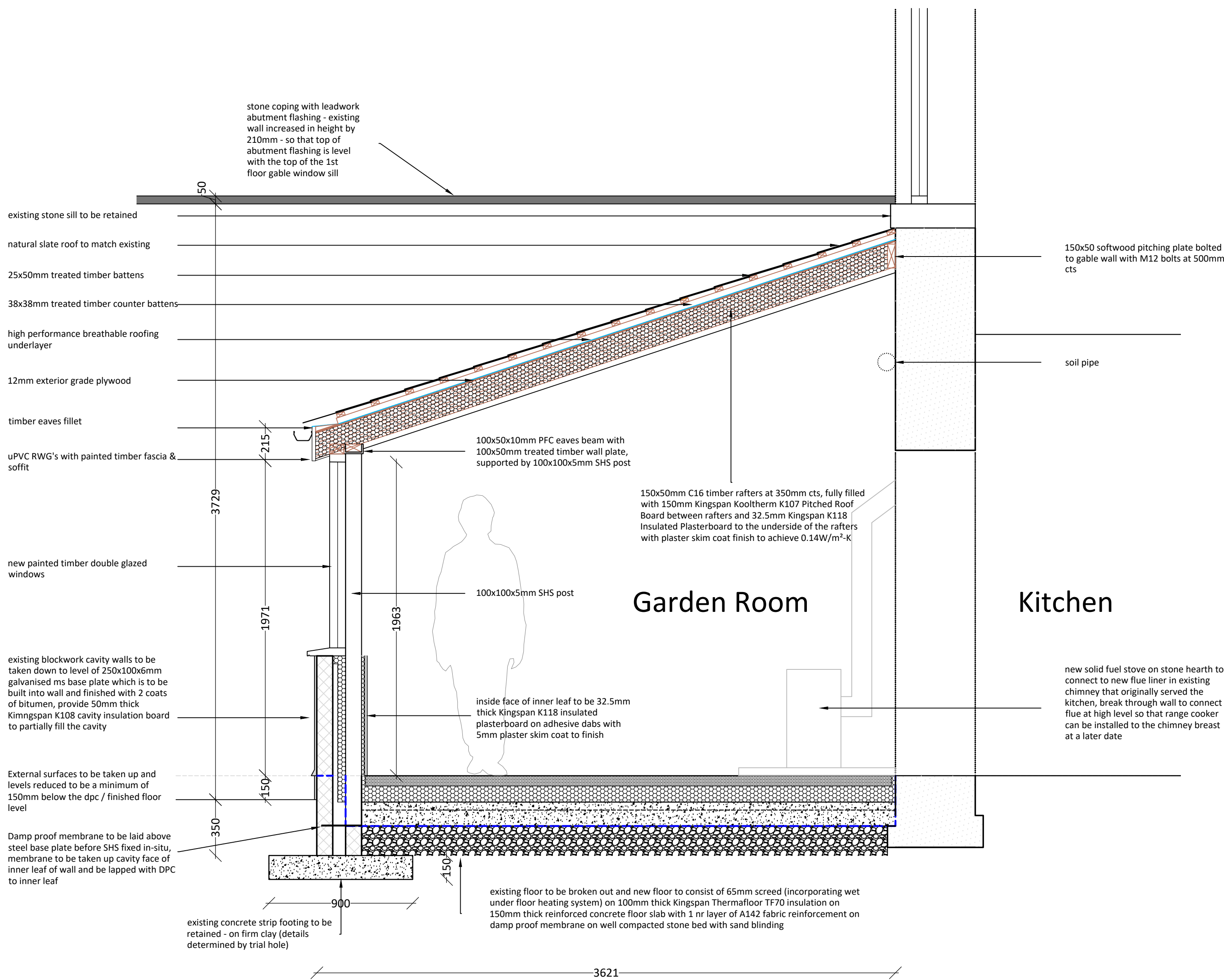
PROPOSED SECTION A-A 1: 20 @ A1
