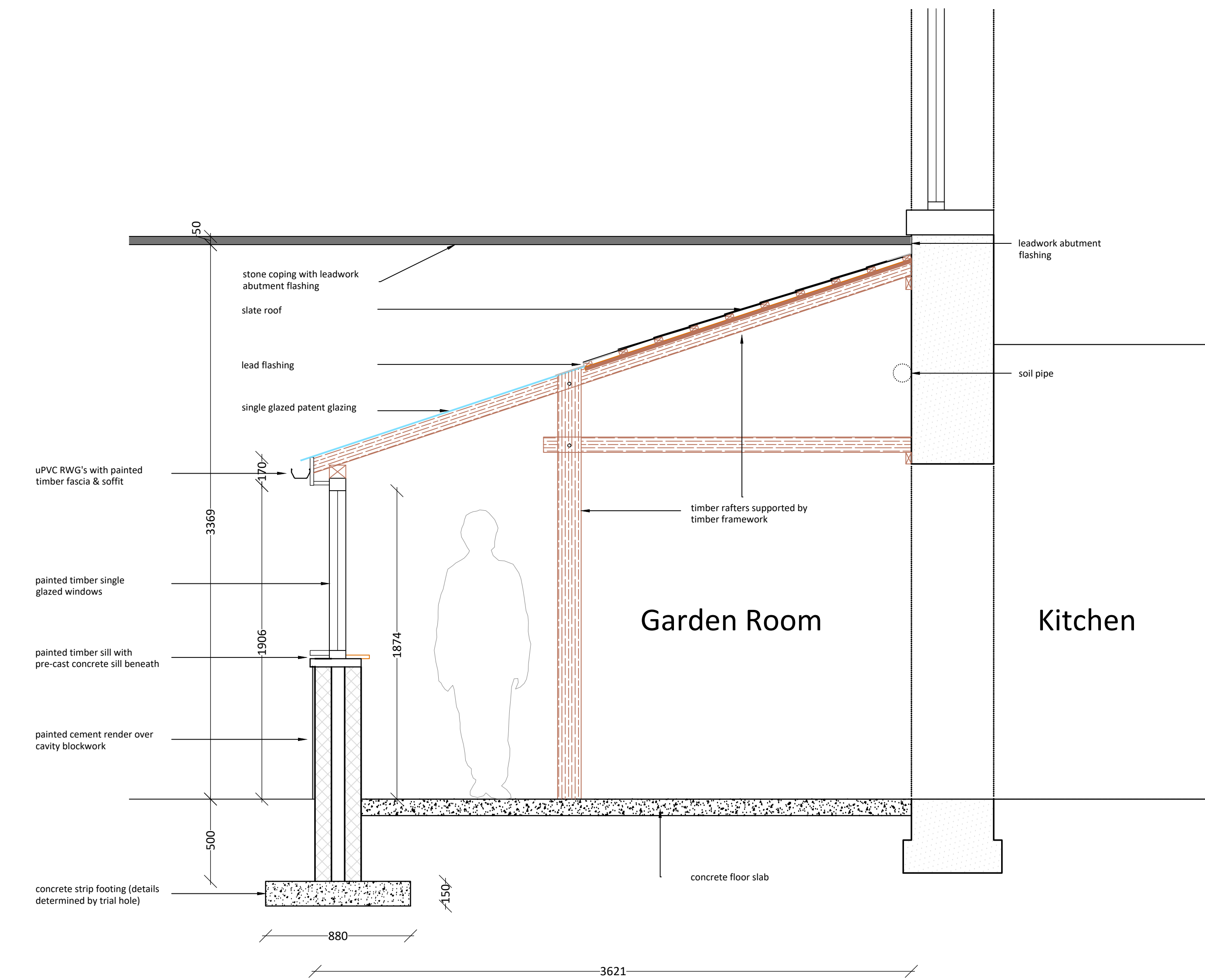
EXISTING SECTION A-A 1: 20 @ A1
