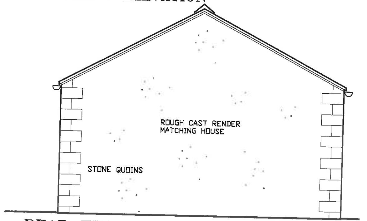
REAR ELEVATION
