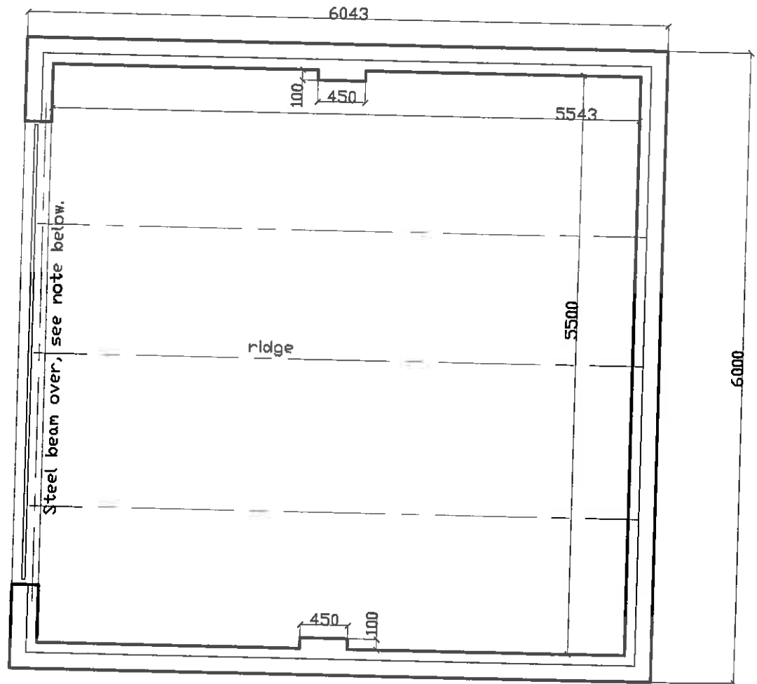
GARAGE PLAN.
