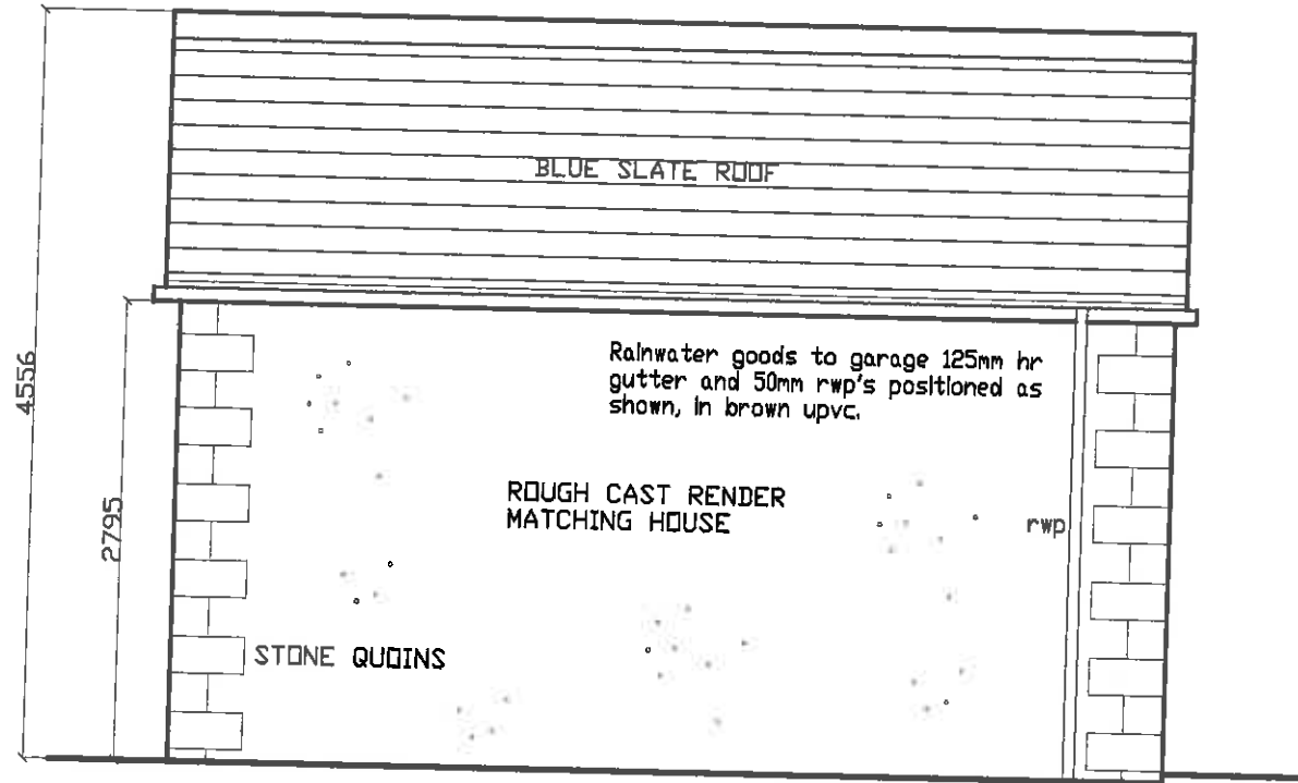
SIDE ELEVATIONS
