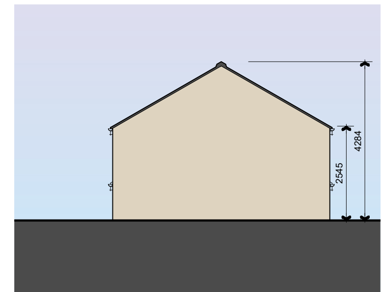
South East Elevation 1:100
