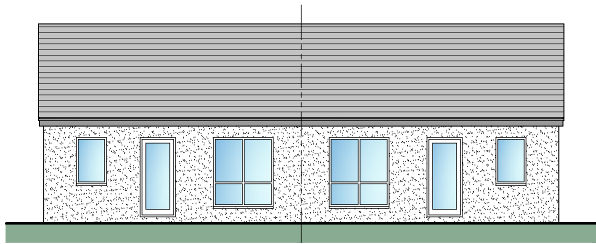
Front Elevation
