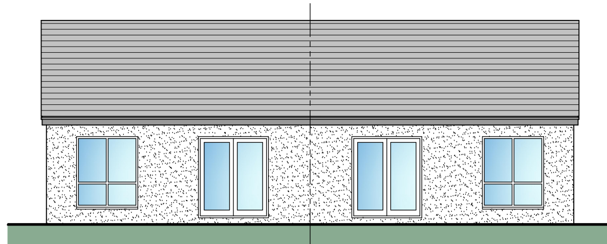
Rear Elevation
