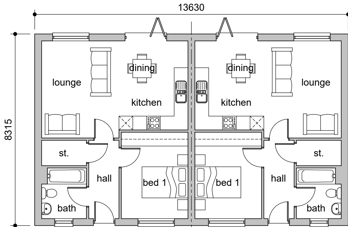
Floor Plan Plot 26 & 27
