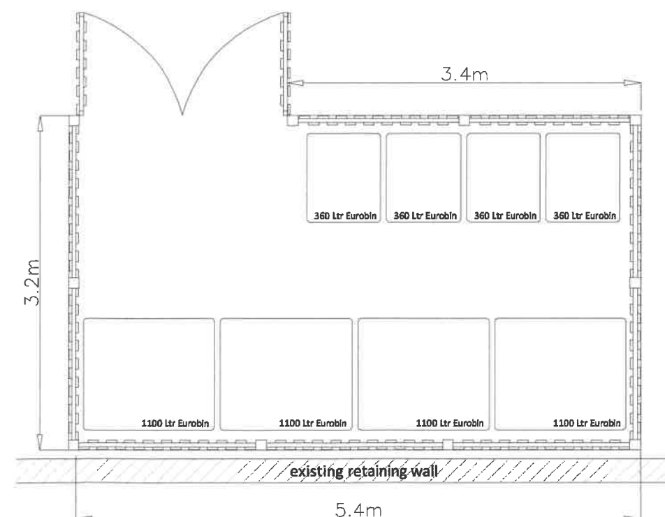
BIN STORE LAYOUT (1:50)
