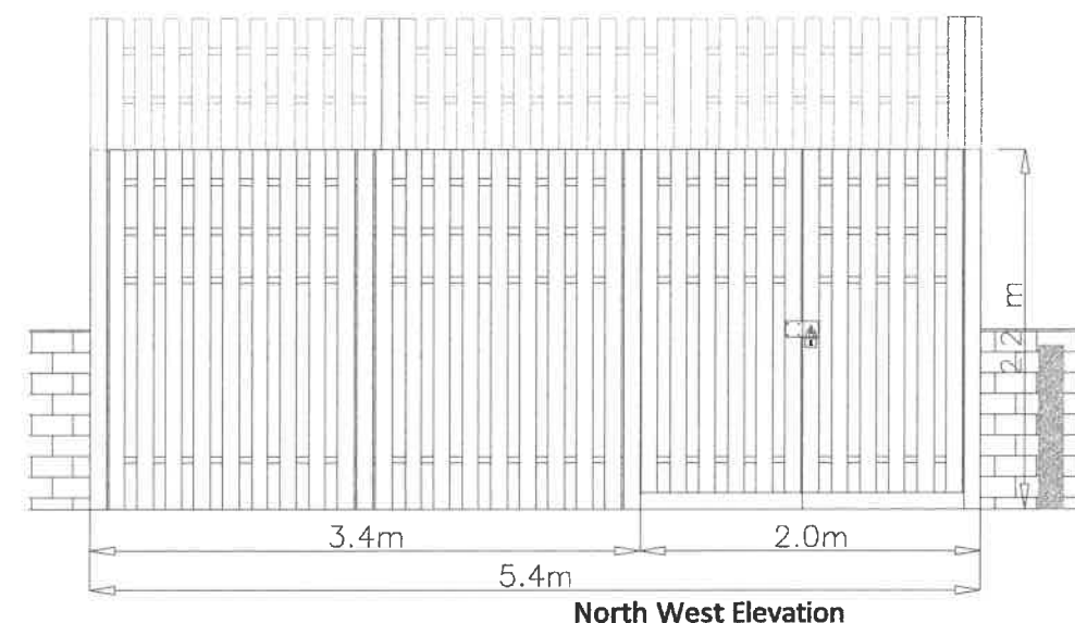
BIN STORE ELEVATIONS (1:50)
