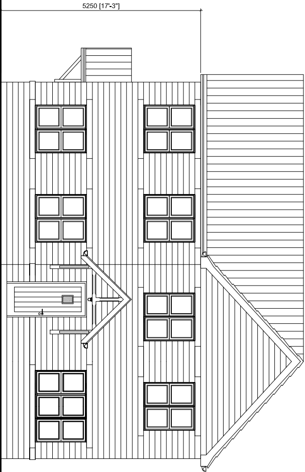
FRONT ELEVATION
