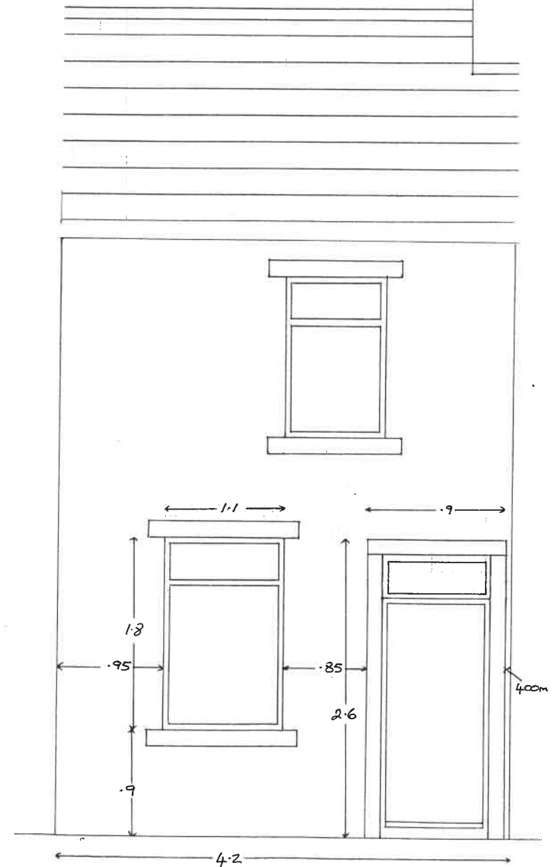
Proposed 1:50
