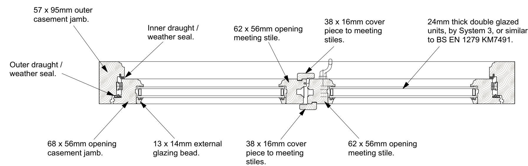
Opening Casement Windows Scale 1:5
