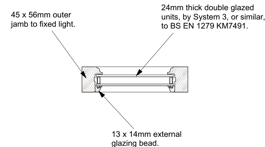
Fixed Casement Windows Scale 1:5
