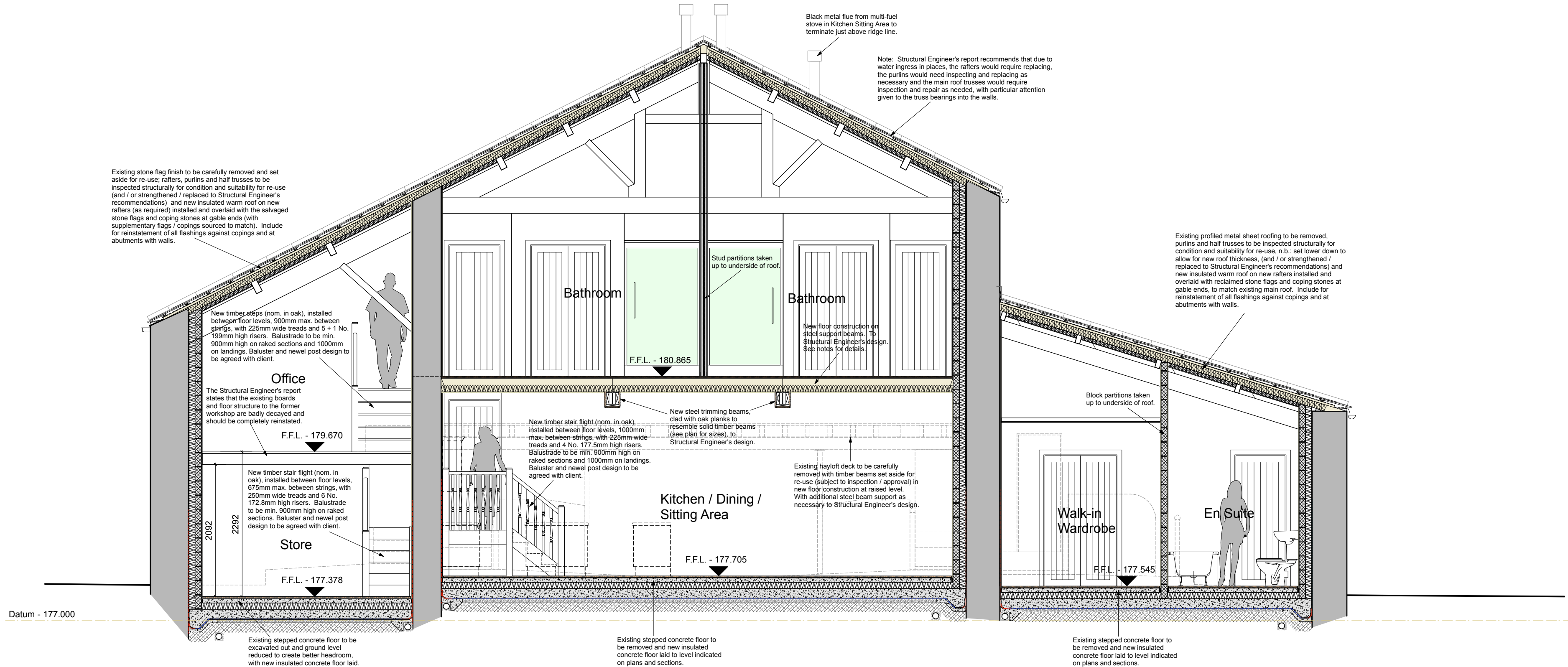
Proposed Section A-A - 1:50
