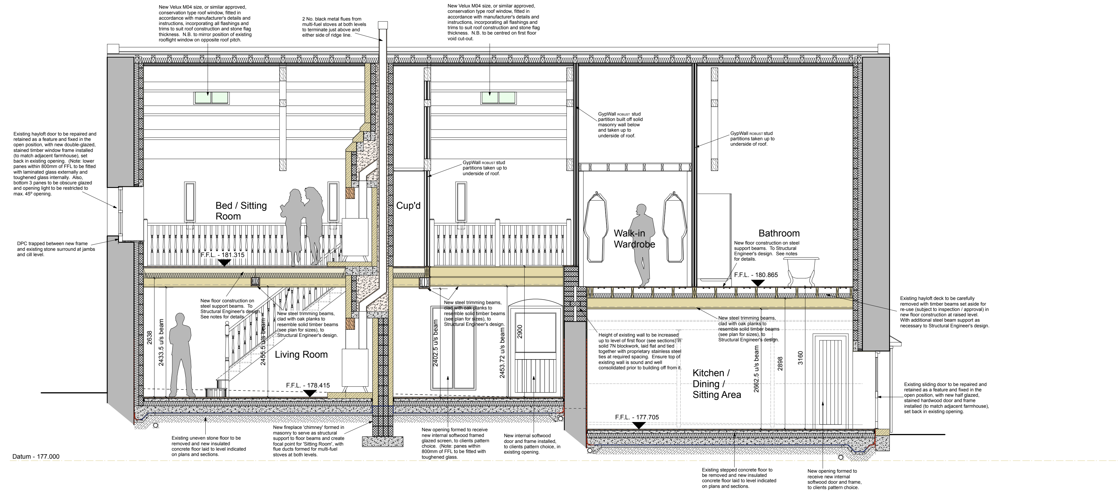
Proposed Section B-B - 1:50
