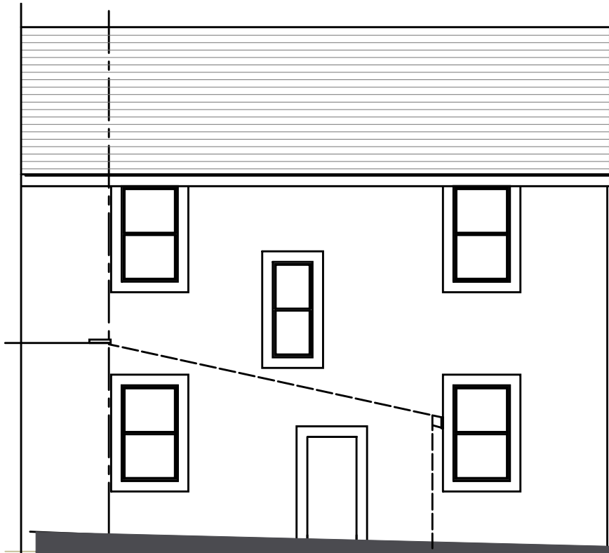
REAR ELEVATION
