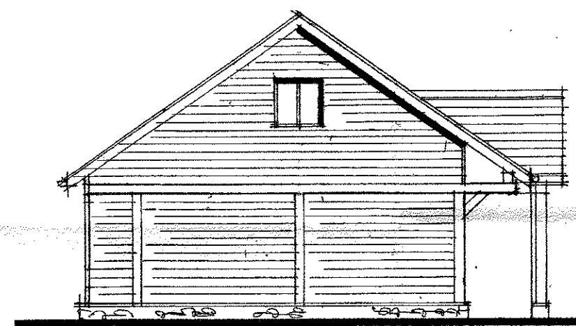
North Elevation
