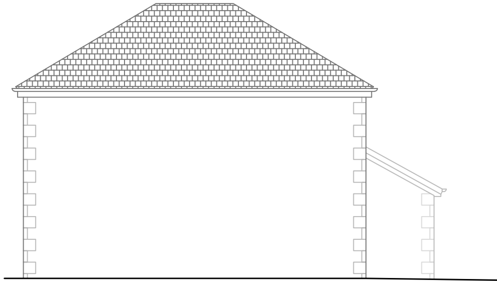
Side Elevation
