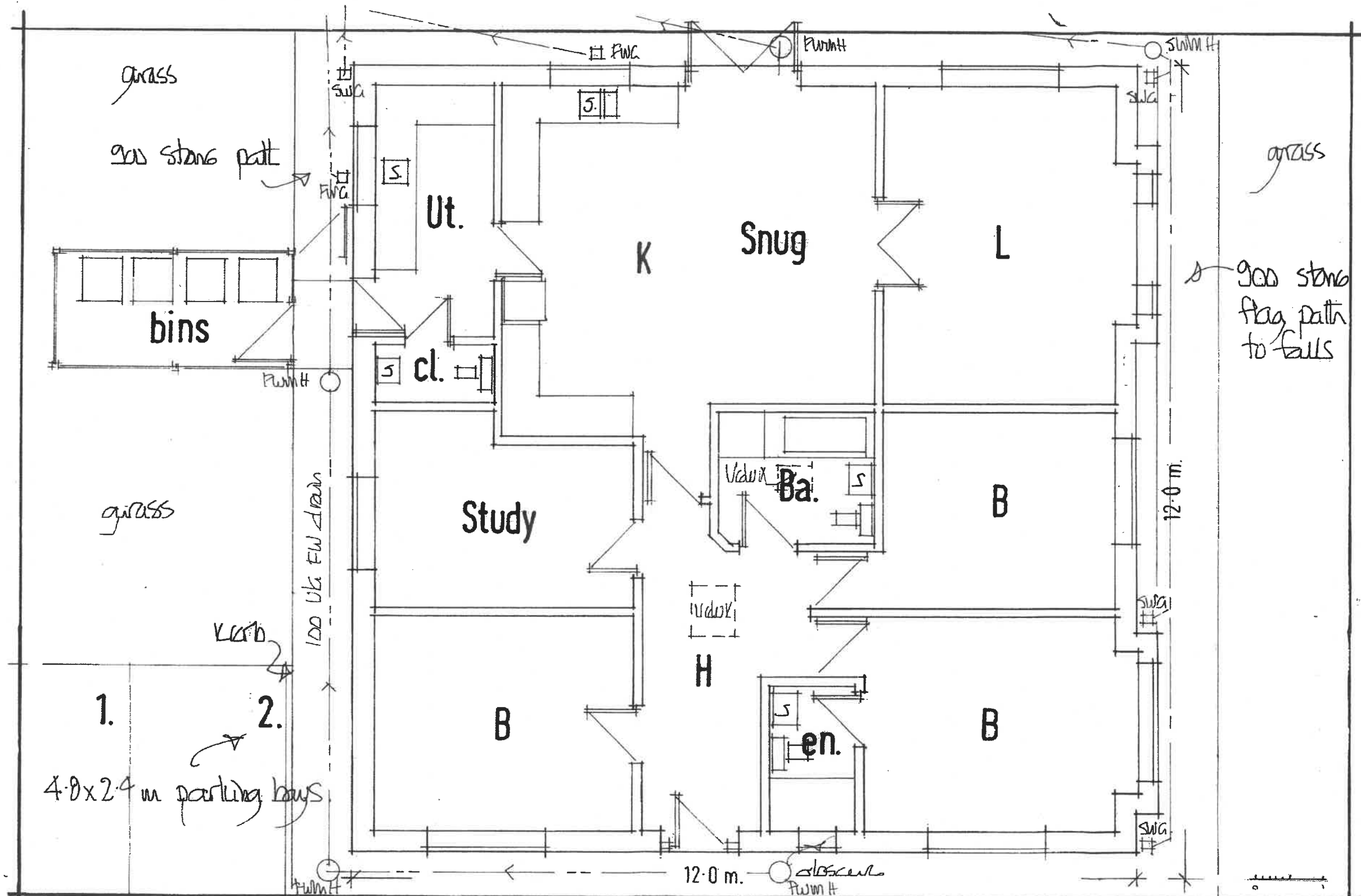
PROPOSED BUNGALOW AT HAWKSHAW FARM, LONGSIGHT ROAD, BB2 7JA. PLAN. 1:50.
