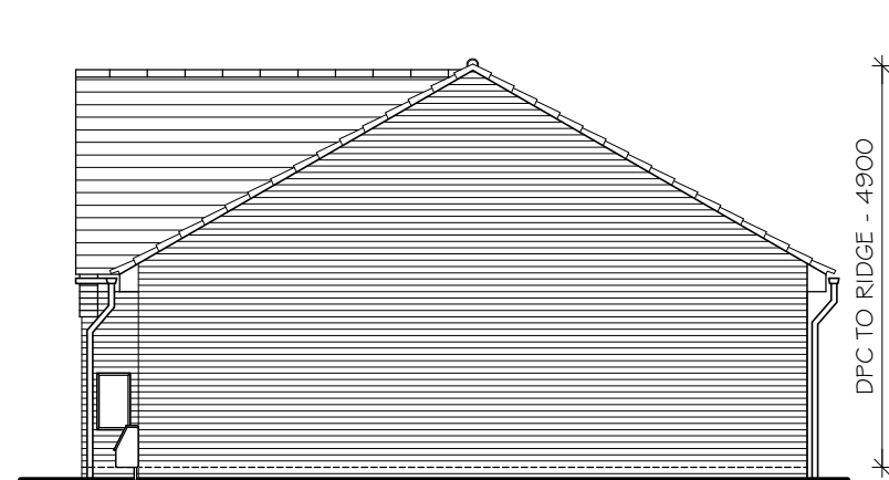
SIDE ELEVATION
