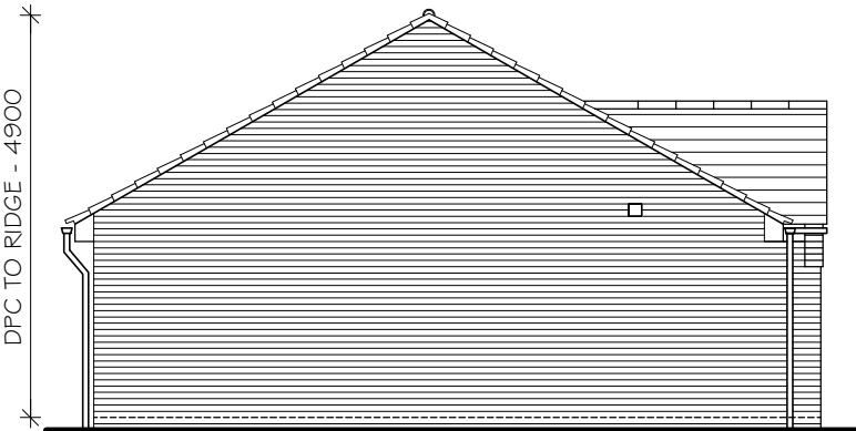
SIDE ELEVATION
