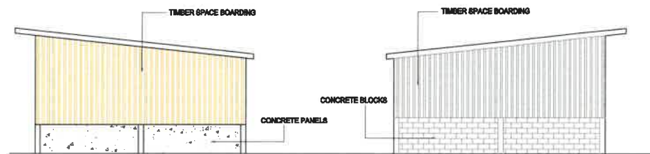
PROPOSED SIDE ELEVATION (North - East)
