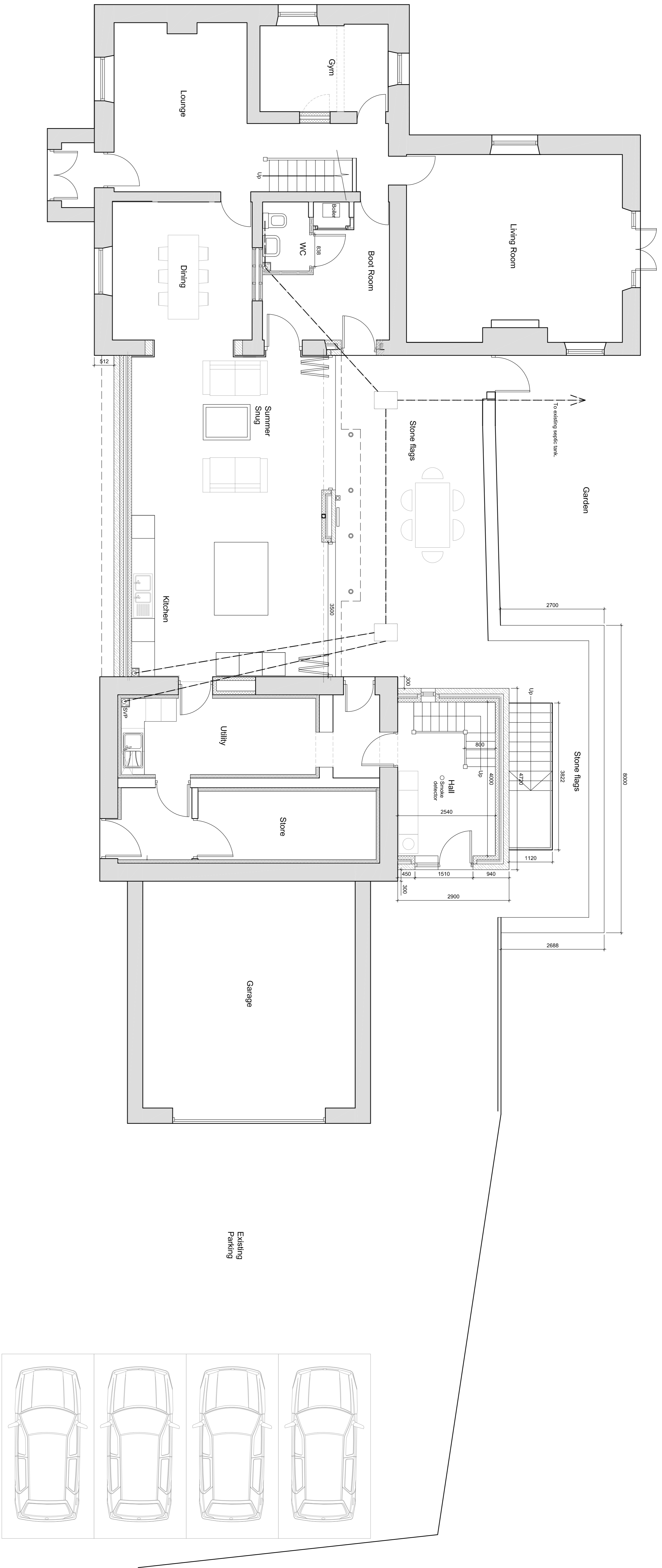
Proposed GF Plan 1:50 Scale
